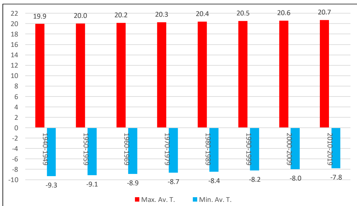
Figure A.14 Decade Average Temperature Trendlines for YQM Since 1940-1949 to 2010-2019
