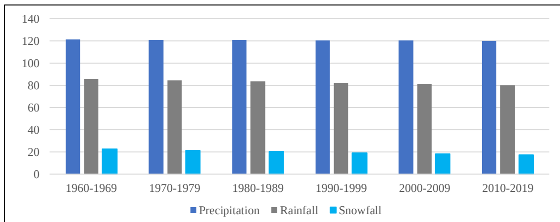
Figure A38 Annual Precip, Rainfall, and Snowfall Trends from YHZ from 1960-1969 to 2010-2019
