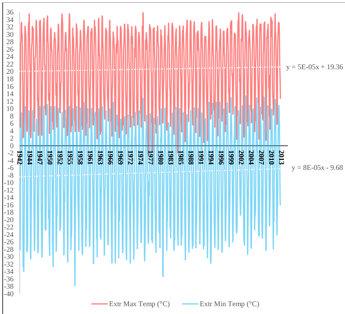
Figure A.5 Monthly Ambient Temperature at YUL from 1942 to 2013
