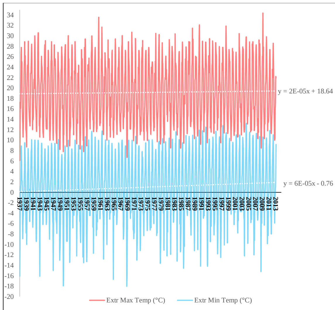
Figure A.3 Monthly Ambient Temperature at YVR from 1937 to 2013
