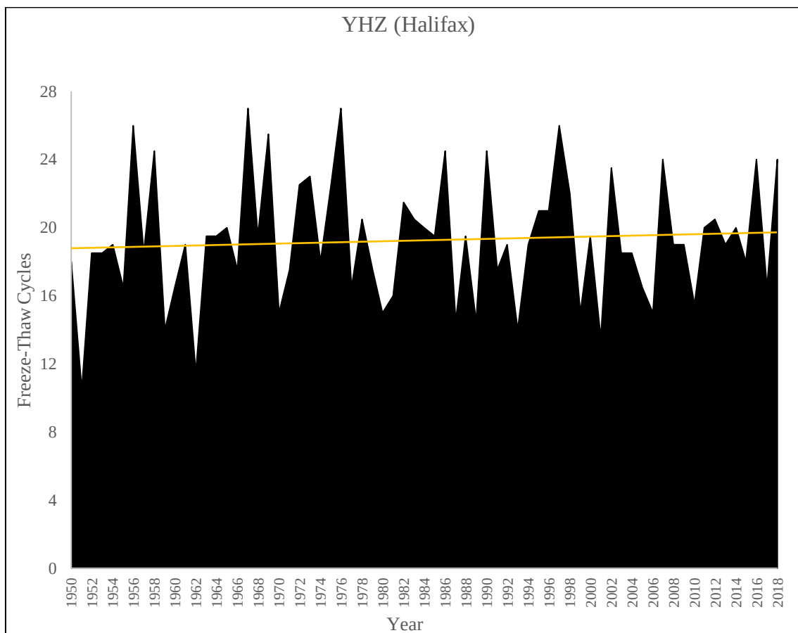
Figure A.30 Annual Freeze-Thaw Cycles for Halifax Stanfield International Airport
