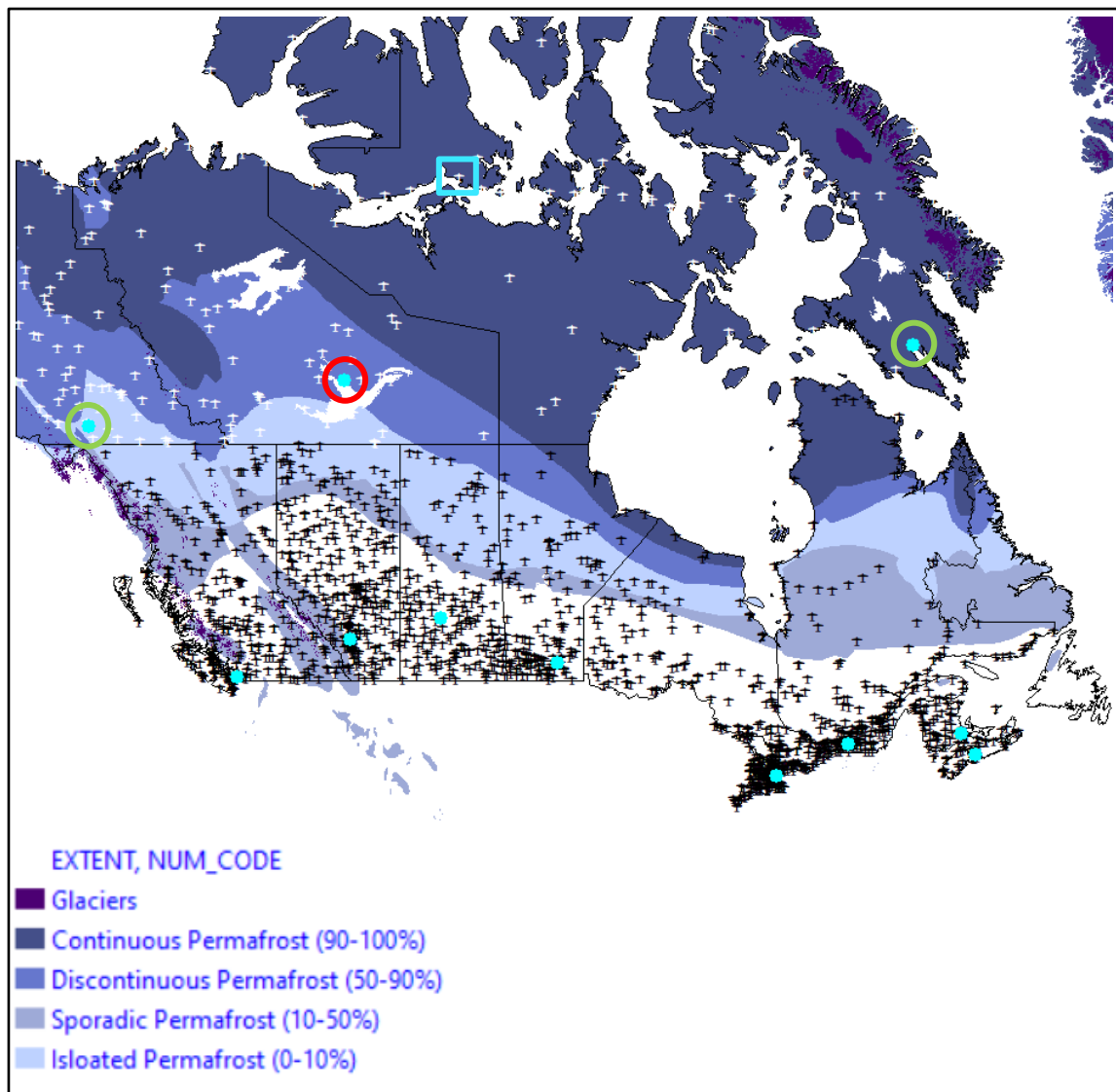
Figure 4.13 Permafrost Composition and Inequality at the Selected Airports (Bone, 2019)
