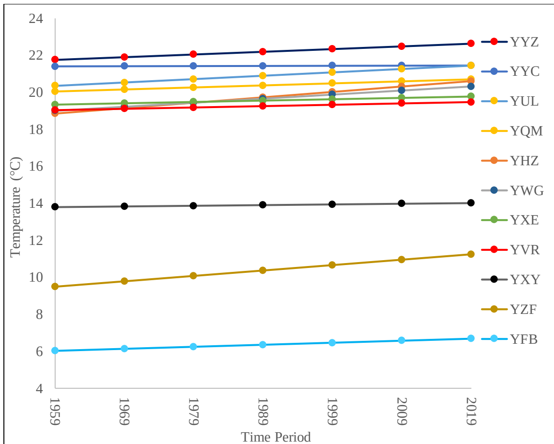
Figure 4.5 Average Maximum Temperature Trendlines
