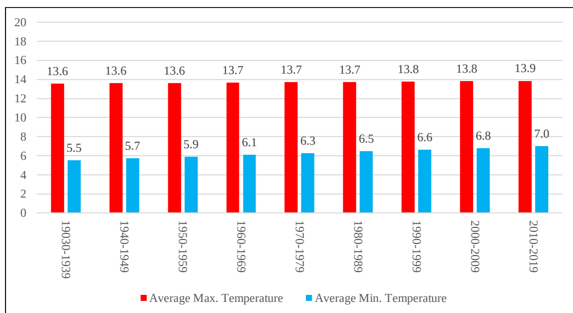
Figure A.4 Decade Average Temperature Trendlines for YVR from 1930-1939 to 2010-2019
