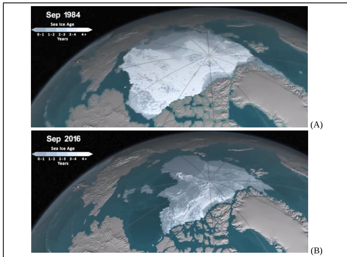
Image 2.1 Arctic Sea Ice Reduction from Sep 1984 to Sep 2016 | A. 1984; B. 2016 (NASA, 2016)
