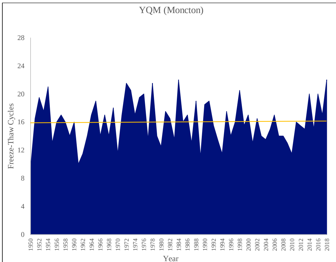
Figure A.28 Annual Freeze-Thaw Cycles for Moncton International Airport
