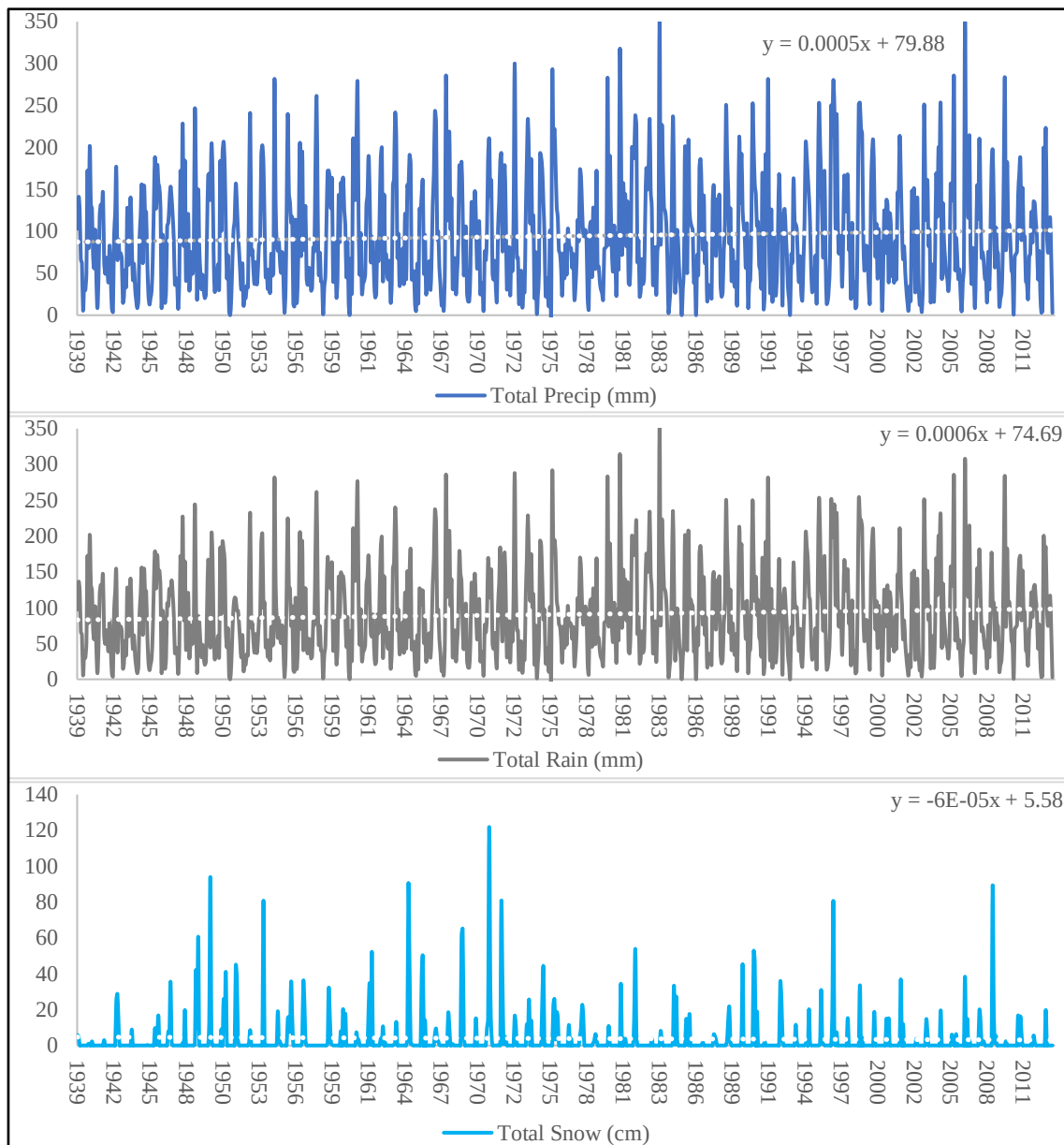
Figure A33 Annual Precipitation, Rainfall, and Snowfall for YVR from 1939 to 2011
