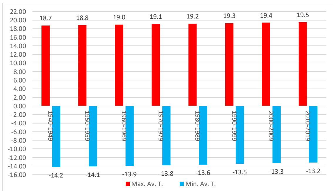
Figure A.12 Decade Average Temperature Trendlines for YWG Since 1940-1949 to 2010-2019
