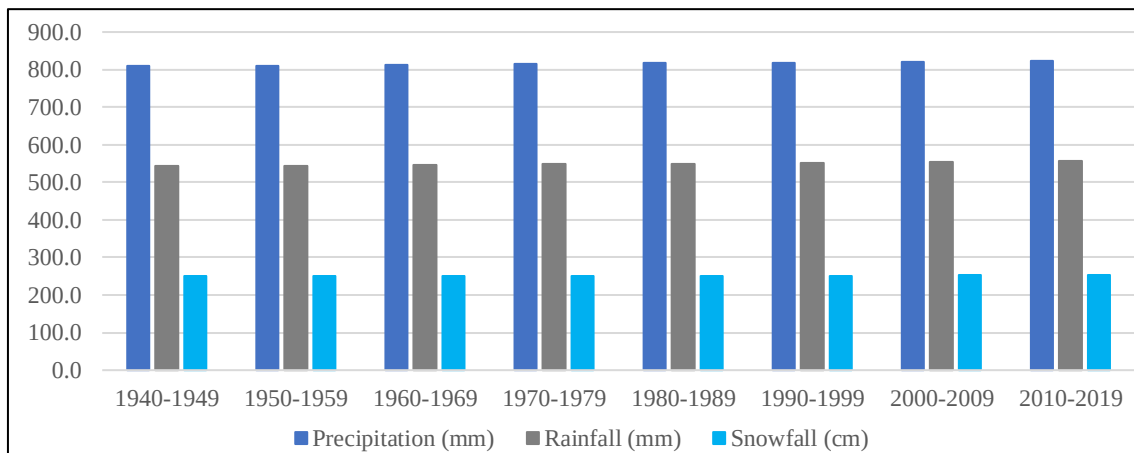
Figure A46 Annual Precip, Rainfall, and Snowfall Trends from YQM from 1940-1949 to 2010-2019
