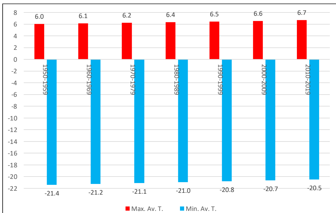
Figure A.20 Decade Average Temperature Trendlines for YFB Since 1950-1959 to 2010-2019
