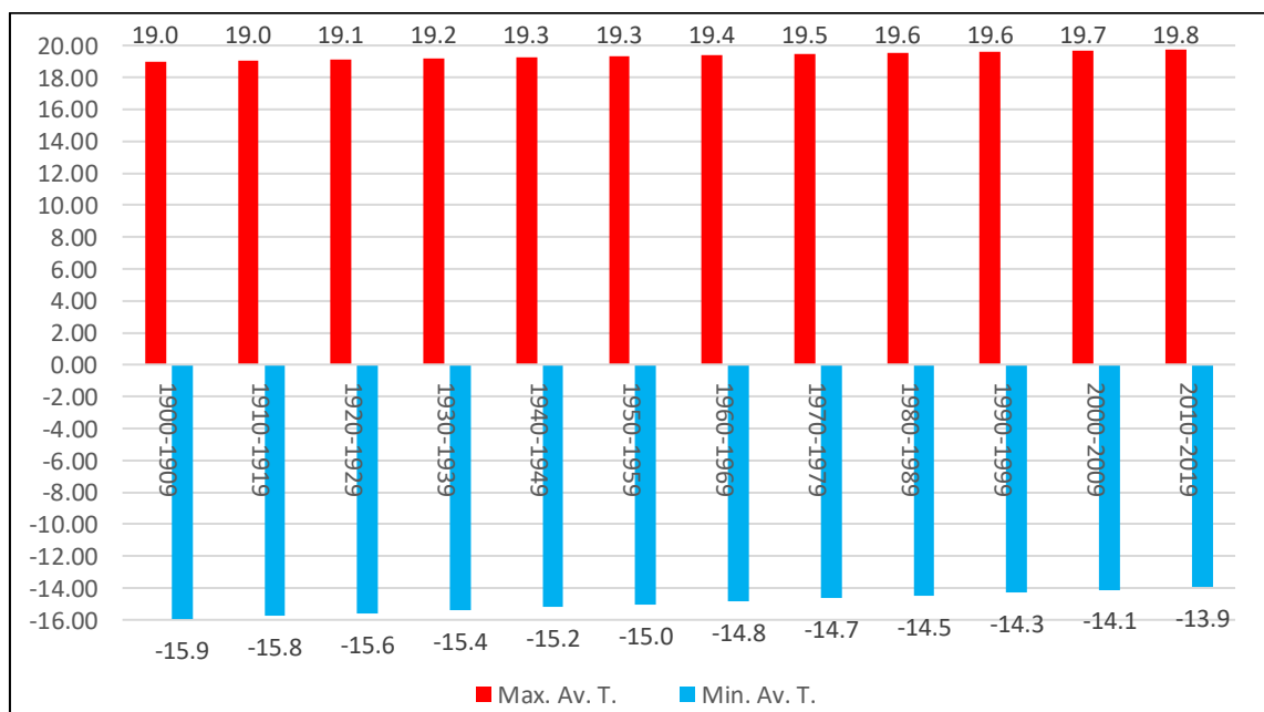
Figure A.10 Decade Average Temperature Trendlines for YXE Since 1900-1909 to 2010-2019
