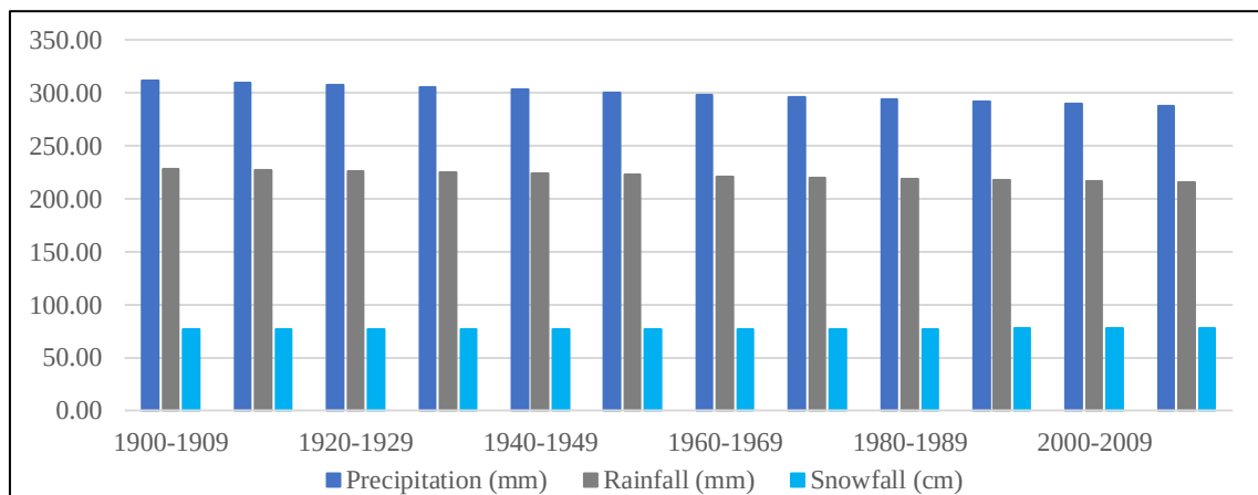
Figure A40 Annual Precip, Rainfall, and Snowfall Trends from YXE from 1900-1909 to 2010-2019
