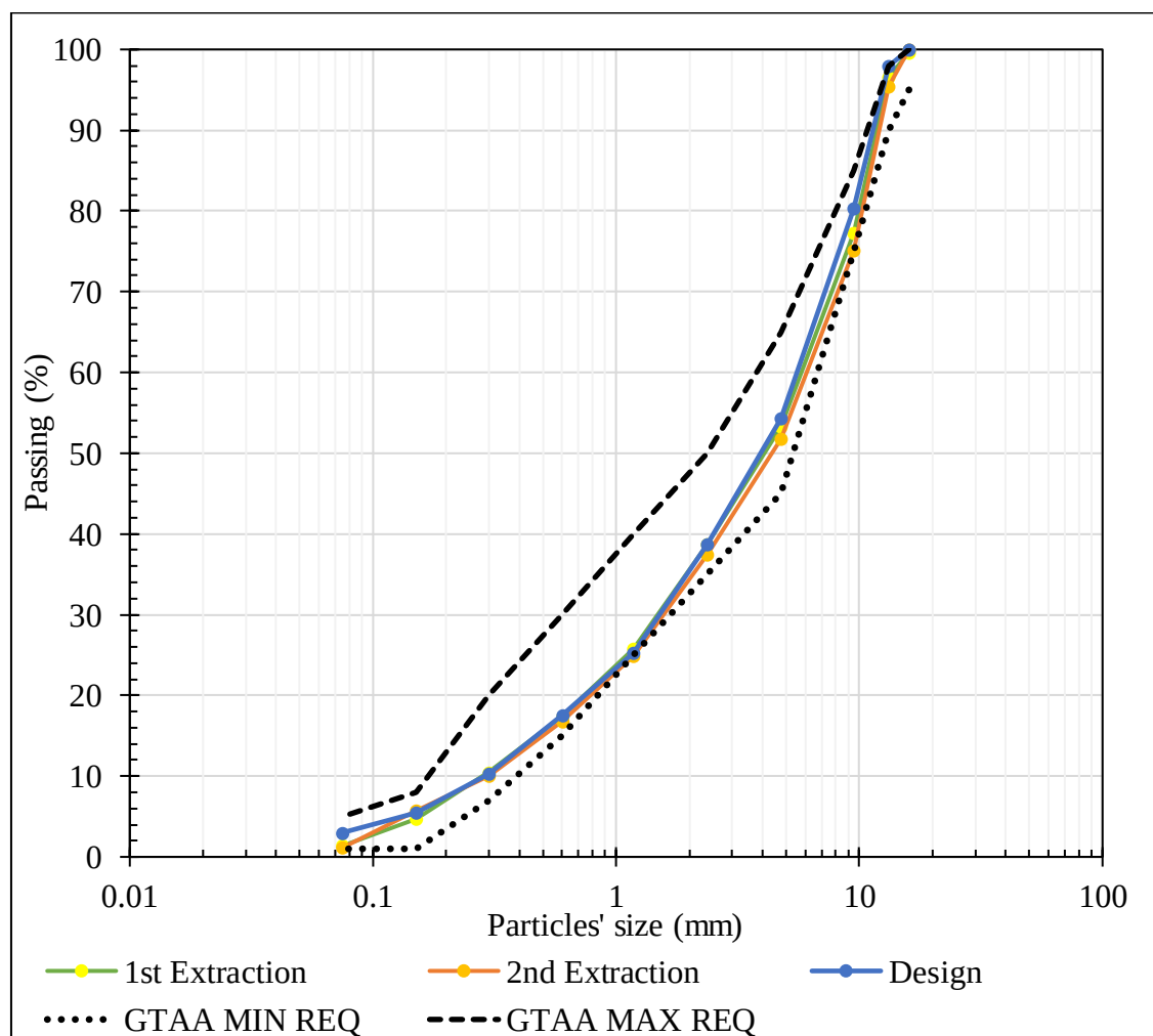
Figure 5.1 Gradation Test's Results
