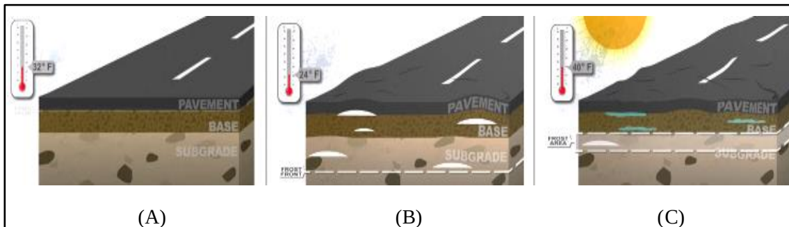
Image 2.6 Frost heaving creation in a flexible pavement | A. New Pavement; B. Frozen Pavement Structure; C. Pavement Structure after Thawing (Minnesota Department of Transportation, 2013)
