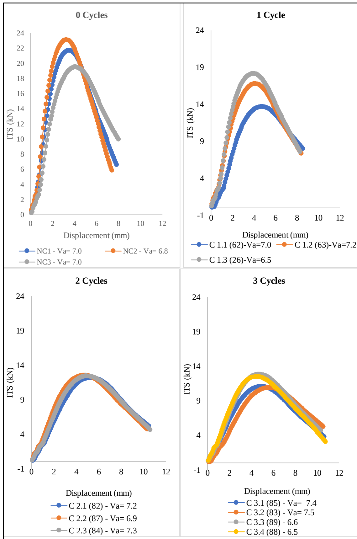
Figure B.3 ITS versus Displacement Variations due to F-T Cycles
