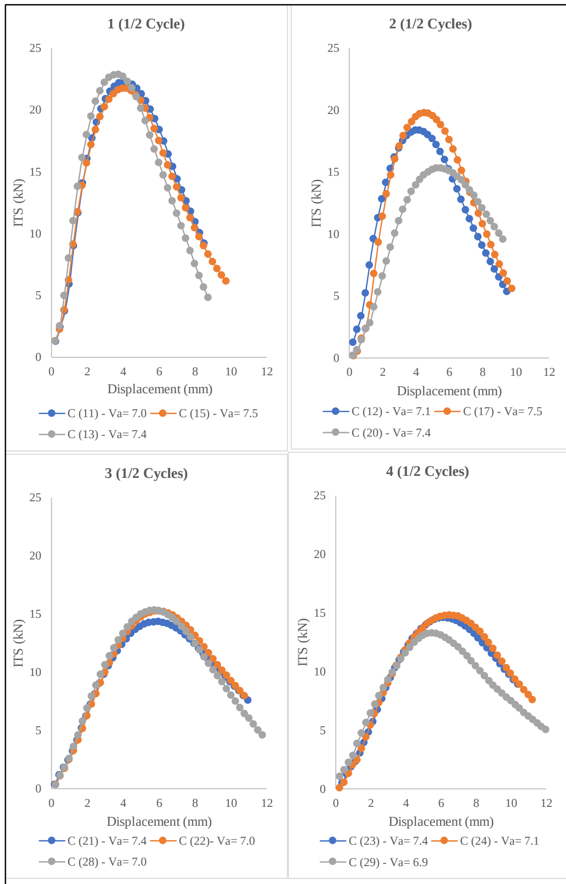
Figure B.5 ITS versus Displacement Variations due to Half F-T Cycles (Higher Speed of Loading)
