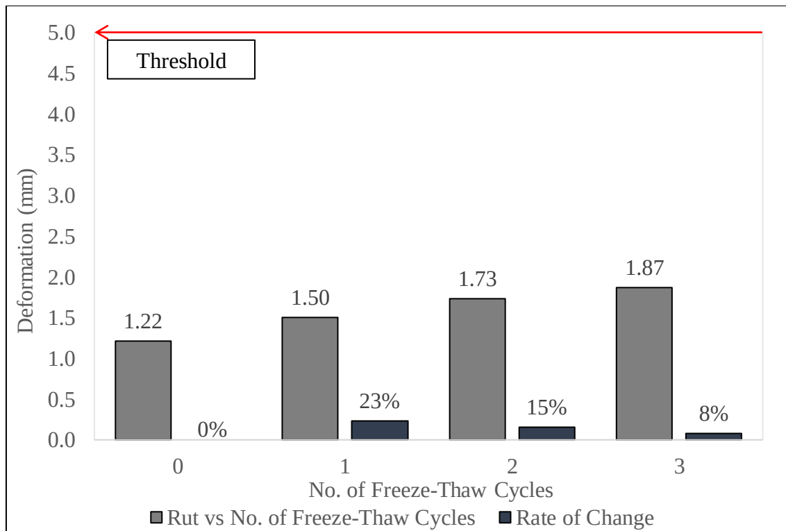
Figure 5.3 Rutting at 10,000-Wheel Passes versus Freeze-Thaw Cycles and Rate of Change
