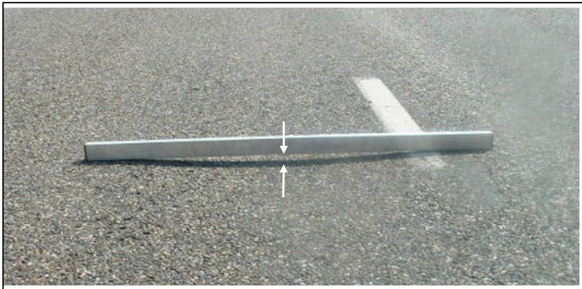
Image 2.5 Moderate Rutting (PPRA, 2018)
