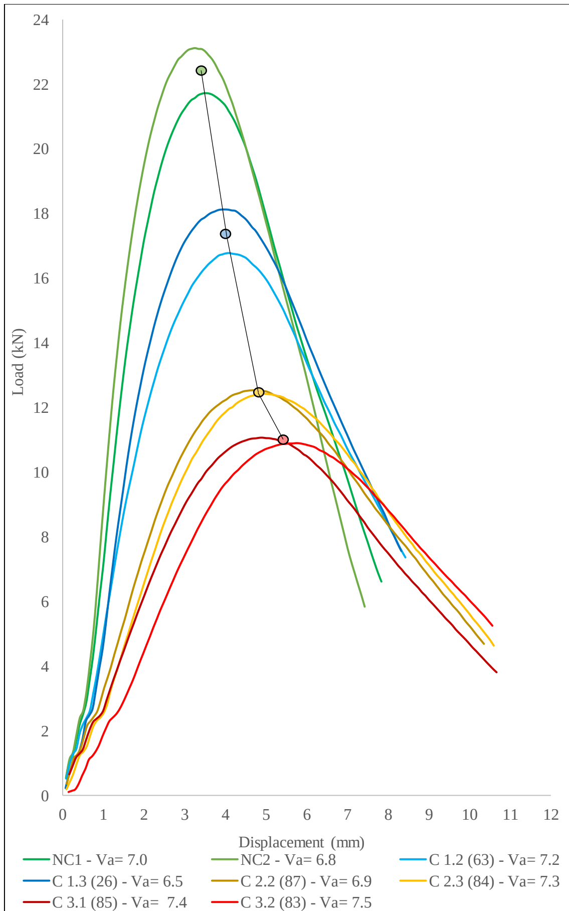
Figure 5.6 Tensile Strength Reduction due to Freeze-Thaw Cycles
