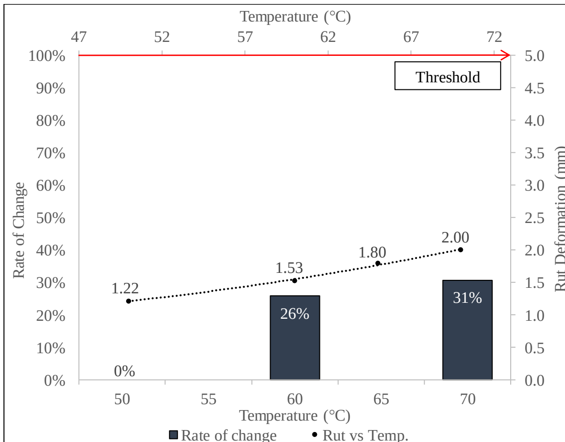
Figure 5.5 Rutting after 10,000 passes versus Temperature and Rate of Change
