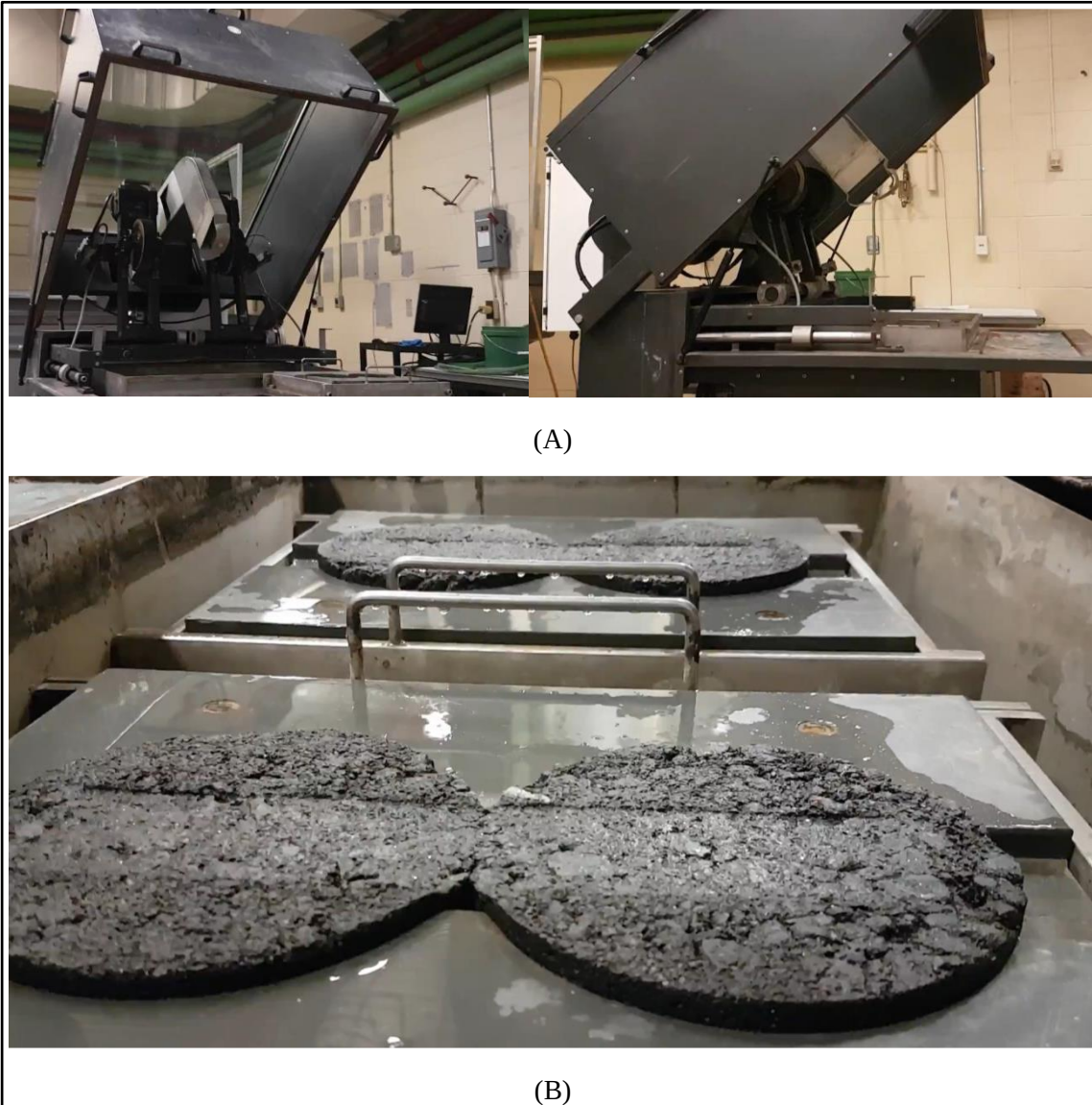
Image 2.10 Hamburg Wheel Tracking Test | A. CPATT's Hamburg Wheel Tracking Device; B. Asphalt Samples inside the HWTDD after Being Tested
