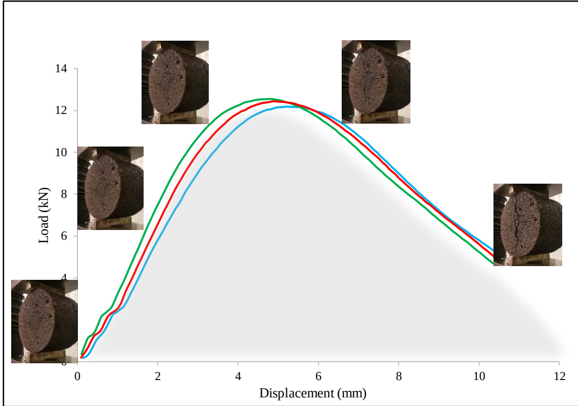
Figure 2.14 Crack Propagation, Ideal CT Principle
