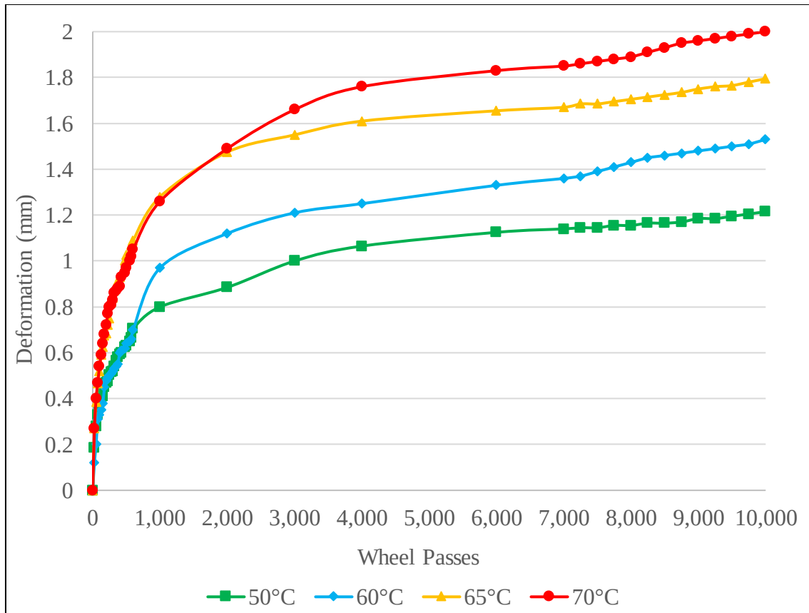
Figure 5.4 Rutting Propagation versus Temperature
