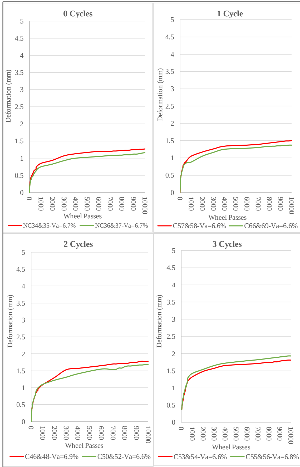
Figure B.2 Rutting Propagation versus Freeze-Thaw Cycles' Variation
