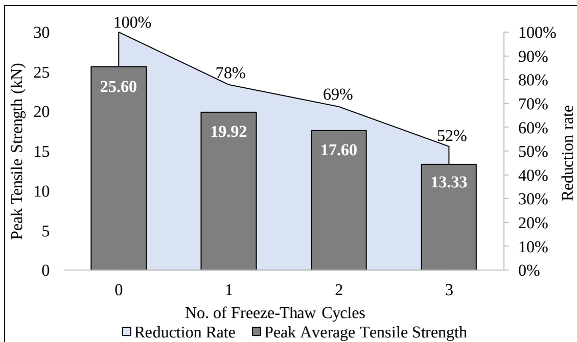
Figure 5.8 Indirect Tensile Strength with Faster Compaction vs Number of Freeze-Thaw Cycles
