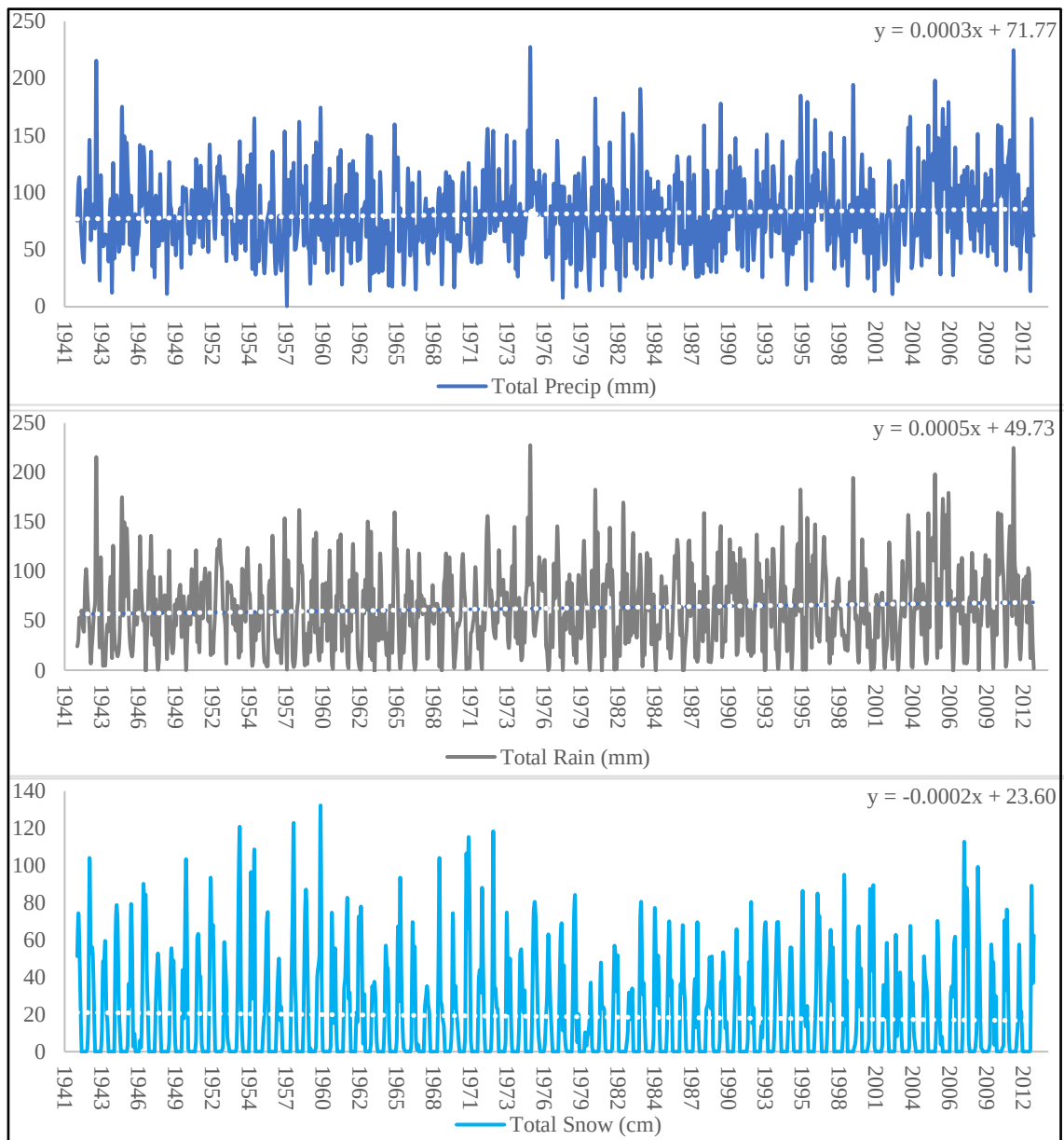
Figure A35 Annual Precipitation, Rainfall, and Snowfall for YUL from 1941 to 2012
