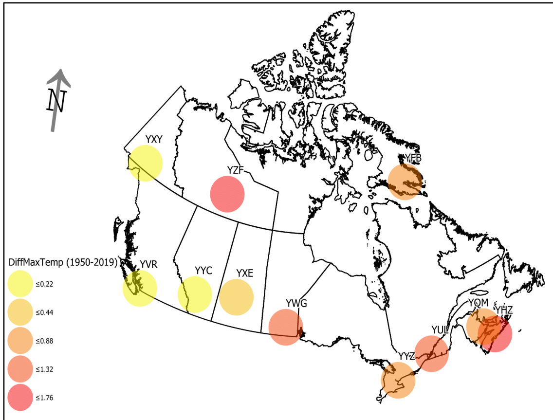
Figure 4.7 Difference in Maximum Temperature Trendlines since 1950
