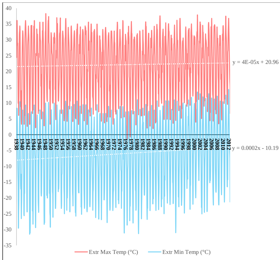
Figure A.1 Monthly Ambient Temperature at YYZ from 1938 to 2012
