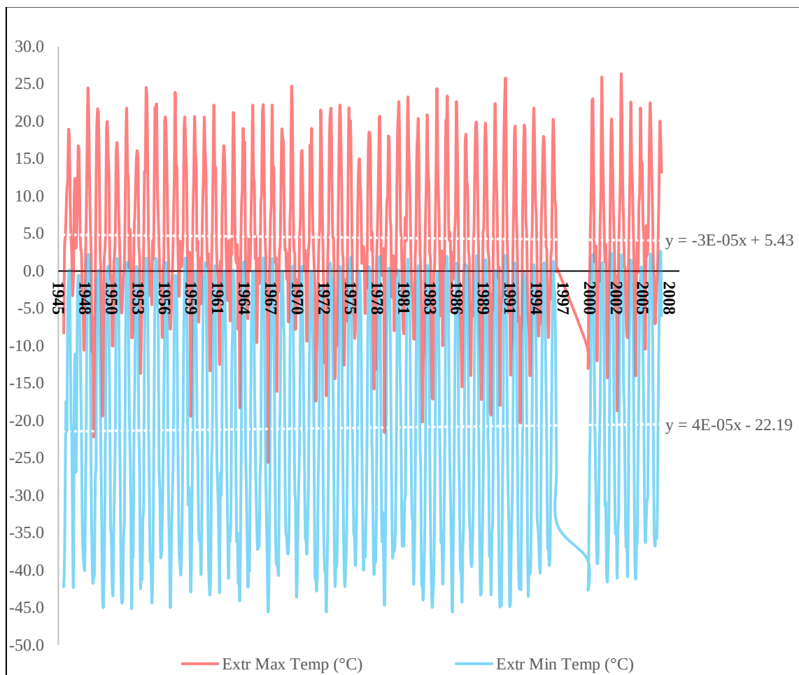
Figure A.19 Monthly Ambient Temperature at YFB from 1945 to 2008
