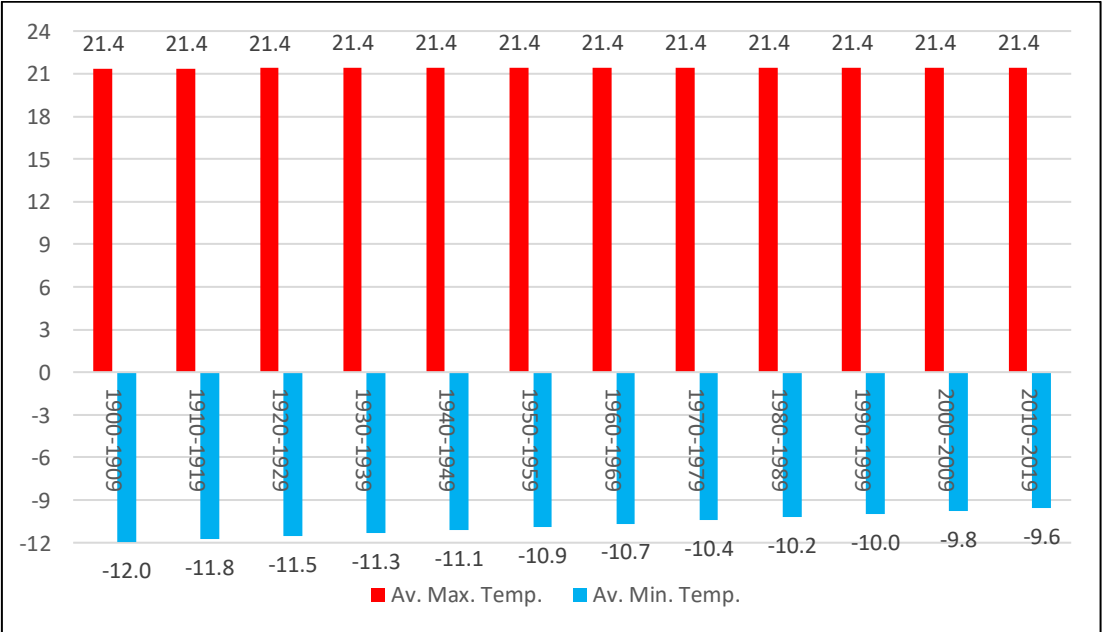
Figure A.10 Decade Average Temperature Trendlines for YYC Since 1900-1909 to 2010-2019
