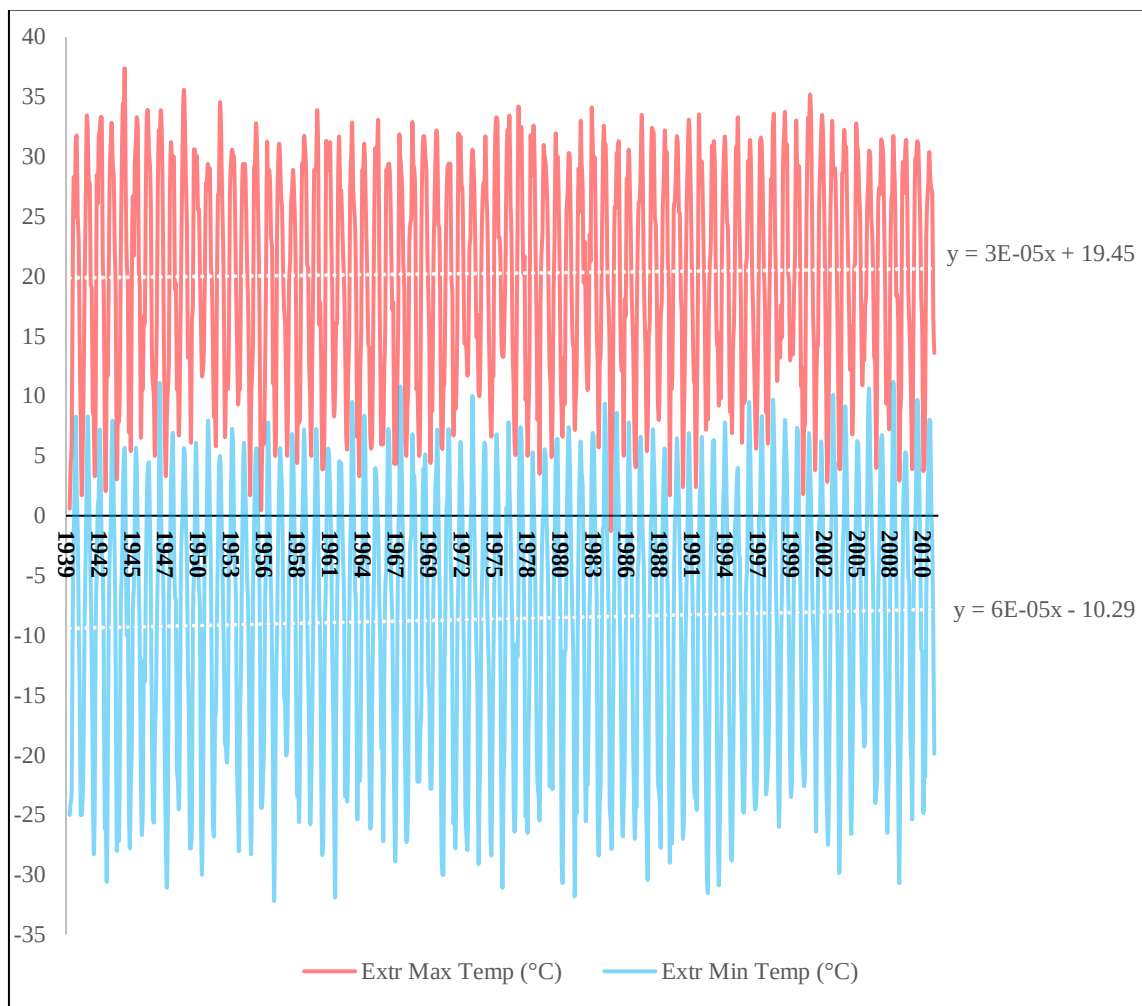
Figure A.13 Monthly Ambient Temperature at YQM from 1939 to 2010
