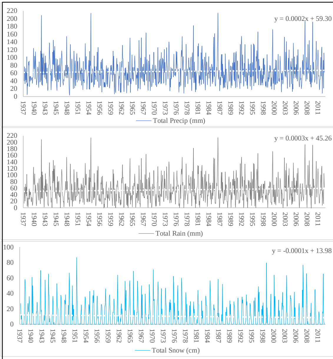
Figure A31 Annual Precipitation, Rainfall, and Snowfall for YYZ from 1937 to 2011
