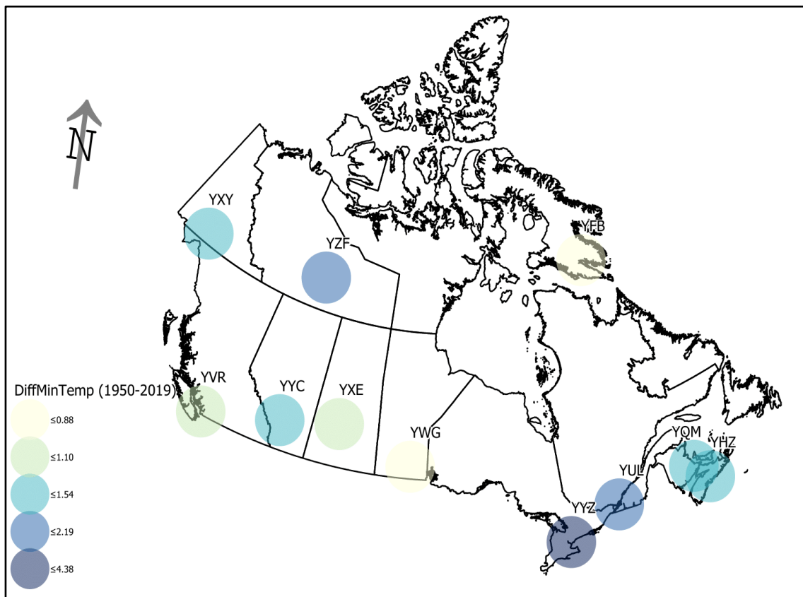
Figure 4.8 Difference in Minimum Temperature Trendlines since 1950
