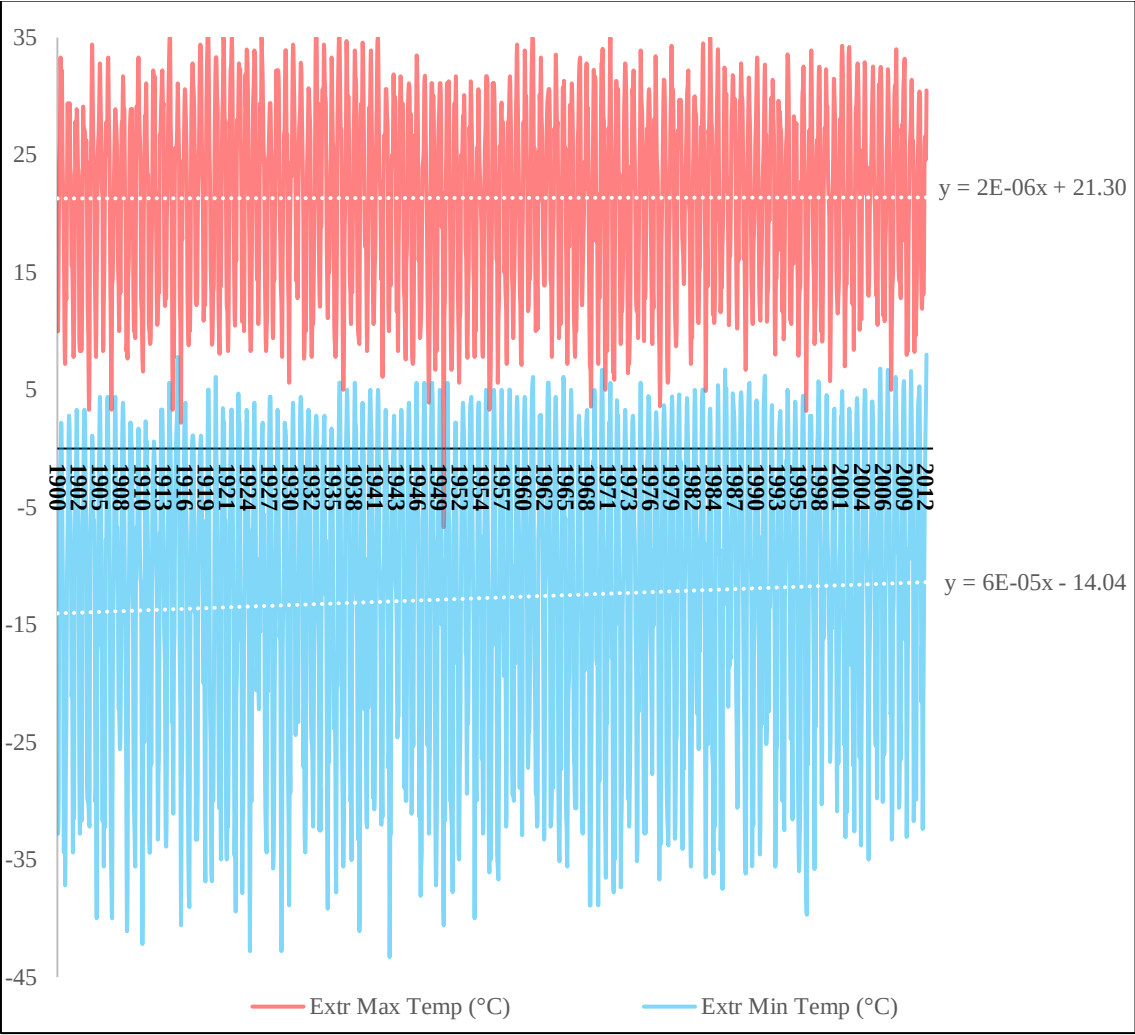
Figure A.9 Monthly Ambient Temperature at YYC from 1900 to 2012
