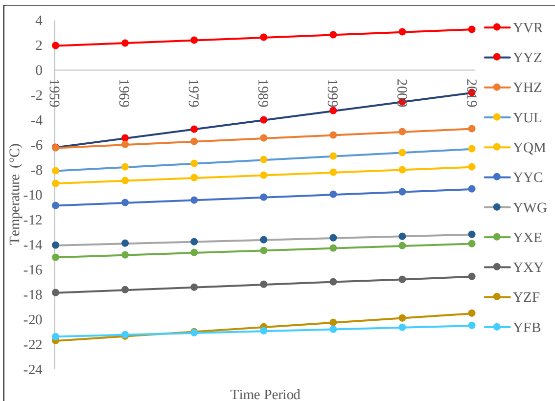
Figure 4.6 Average Minimum Temperature Trendlines
