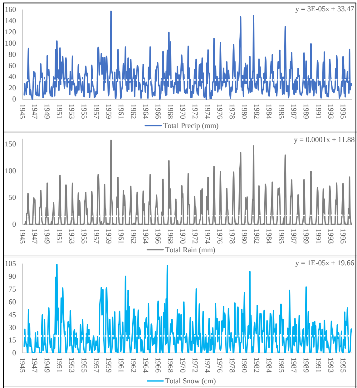
Figure A51 Annual Precipitation, Rainfall, and Snowfall for YFB from 1945 to 1995
