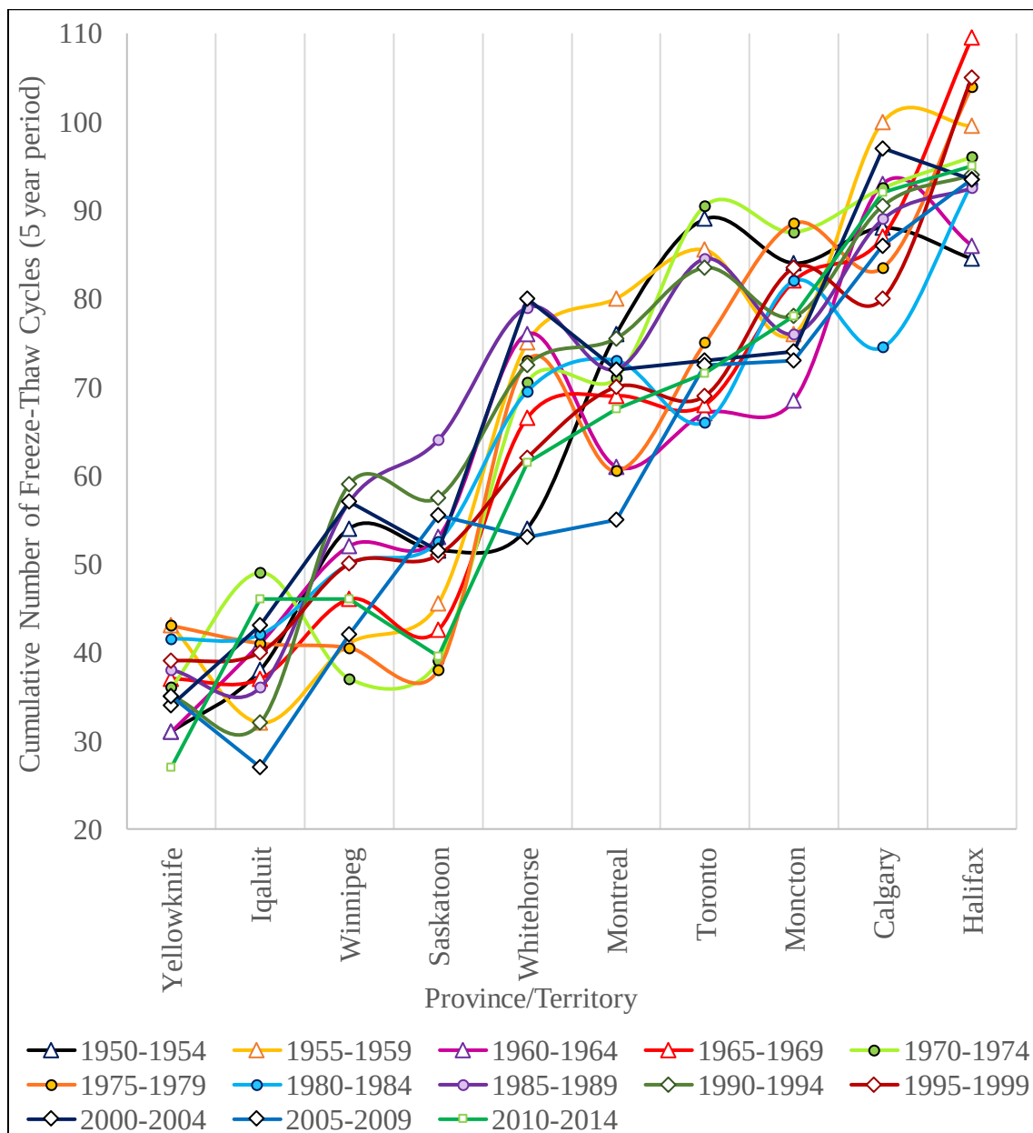
Figure 4.11 Five years Cumulative Annual Freeze-Thaw Cycles at the Selected Airports
