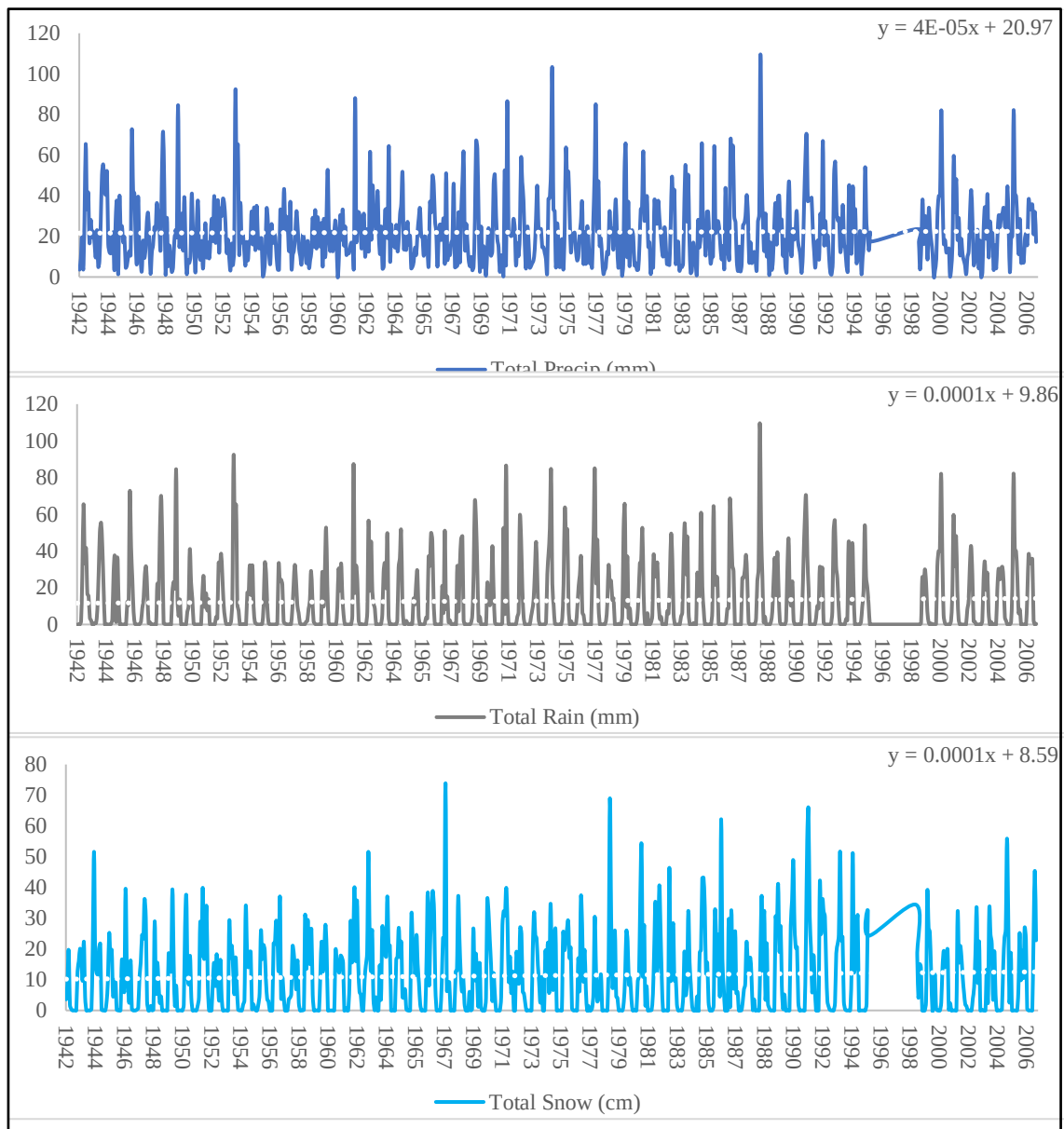
Figure A47 Annual Precipitation, Rainfall, and Snowfall for YXY from 1942 to 2006
