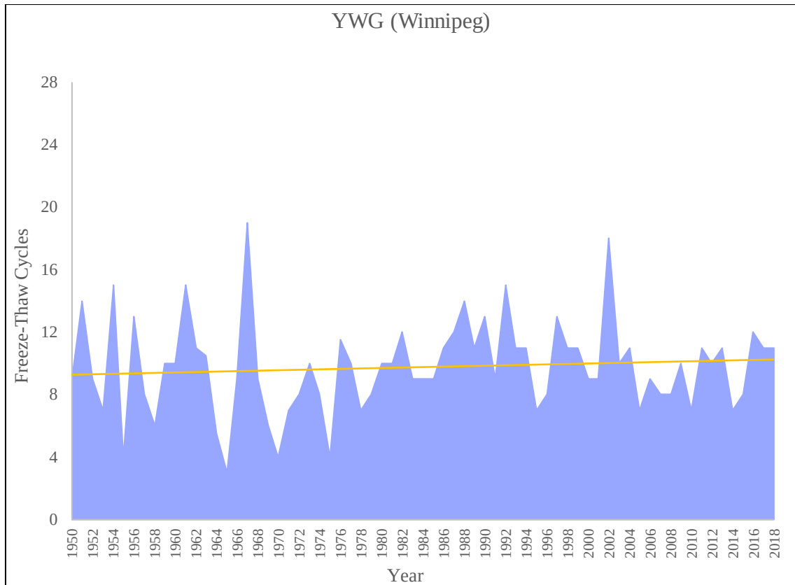
Figure A.23 Annual Freeze-Thaw Cycles for Winnipeg International Airport
