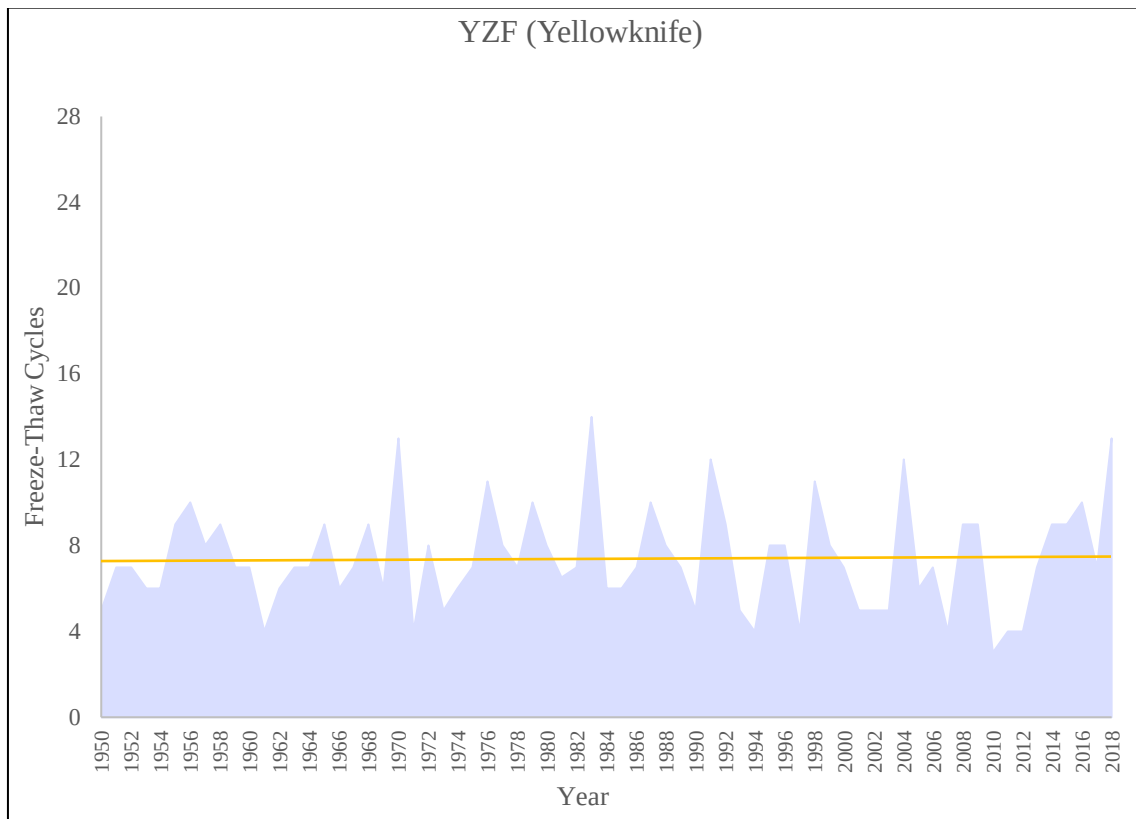
Figure A.21 Annual Freeze-Thaw Cycles for Yellowknife International Airport
