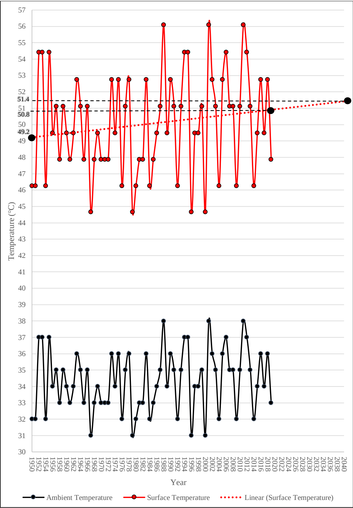
Figure 4.10 Annual Maximum Ambient and Surface Temperatures at YYZ
