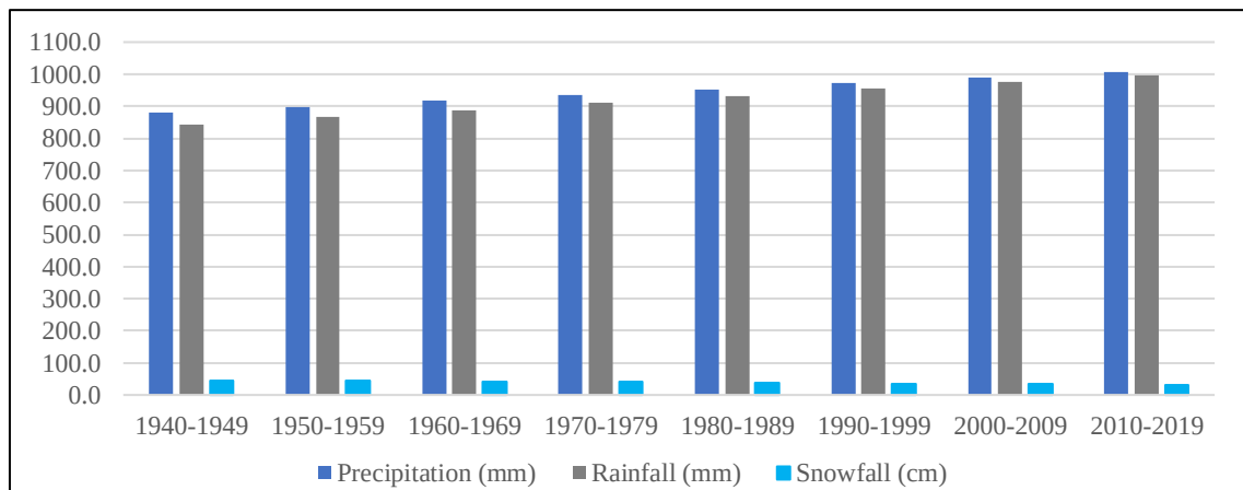
Figure A34 Annual Precip, Rainfall, and Snowfall Trends from YVR from 1940-1949 to 2010-2019
