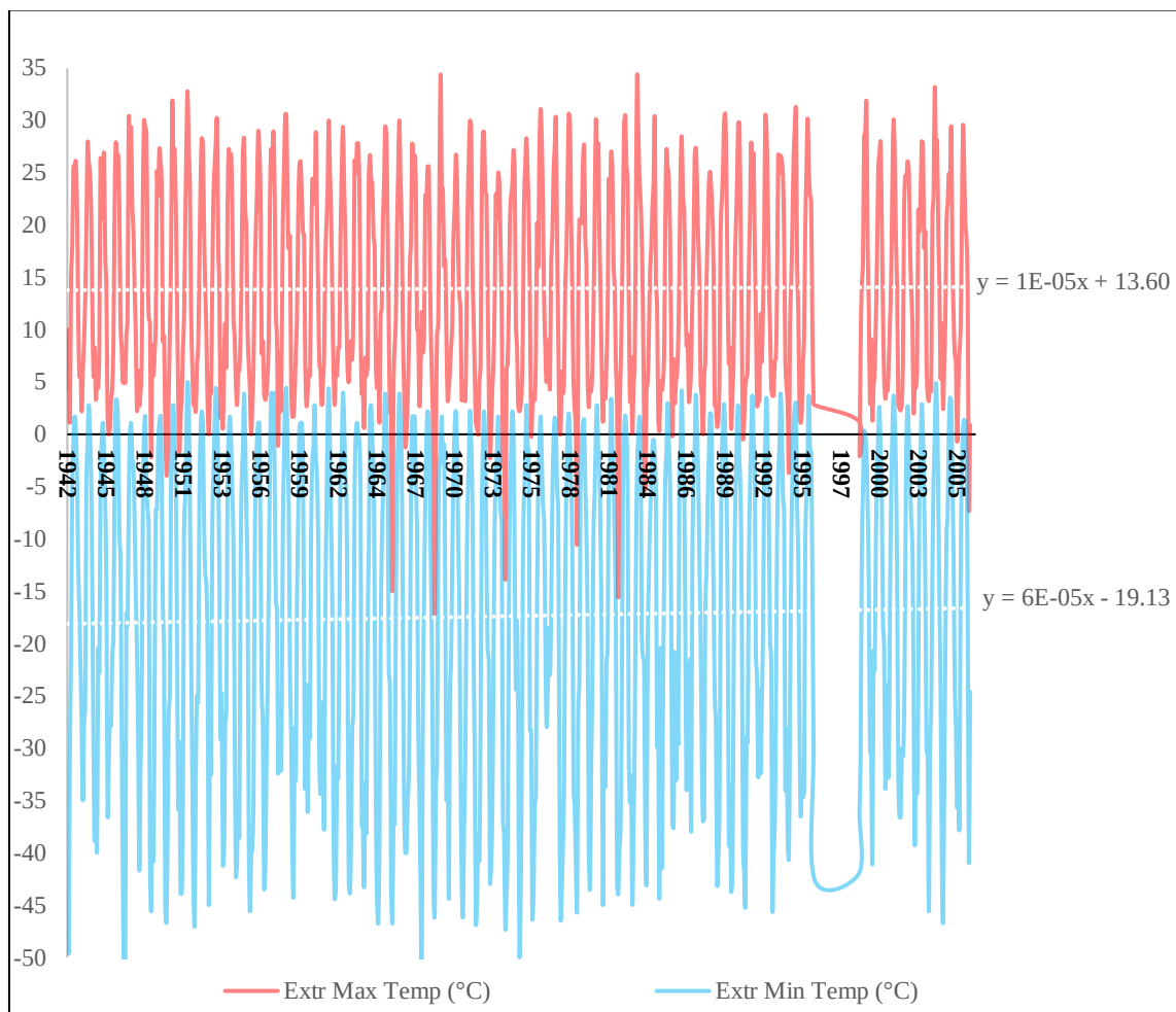
Figure A.15 Monthly Ambient Temperature at YXY from 1942 to 2009
