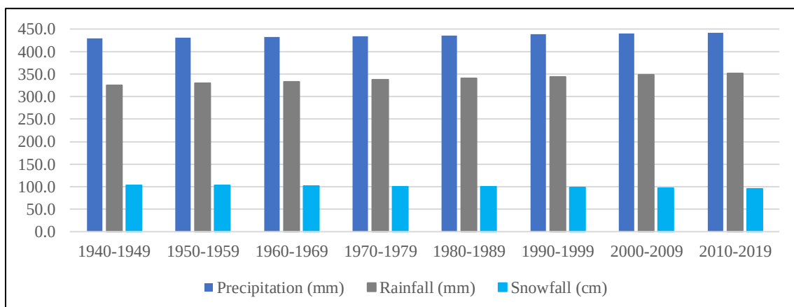
Figure A44 Annual Precip, Rainfall, and Snowfall Trends from YXE from 1940-1949 to 2010-2019
