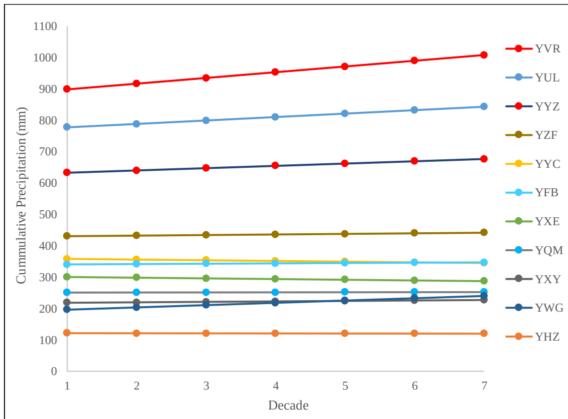
Figure 4.14 Decennial Precipitation at the Selected Airports since 1950
