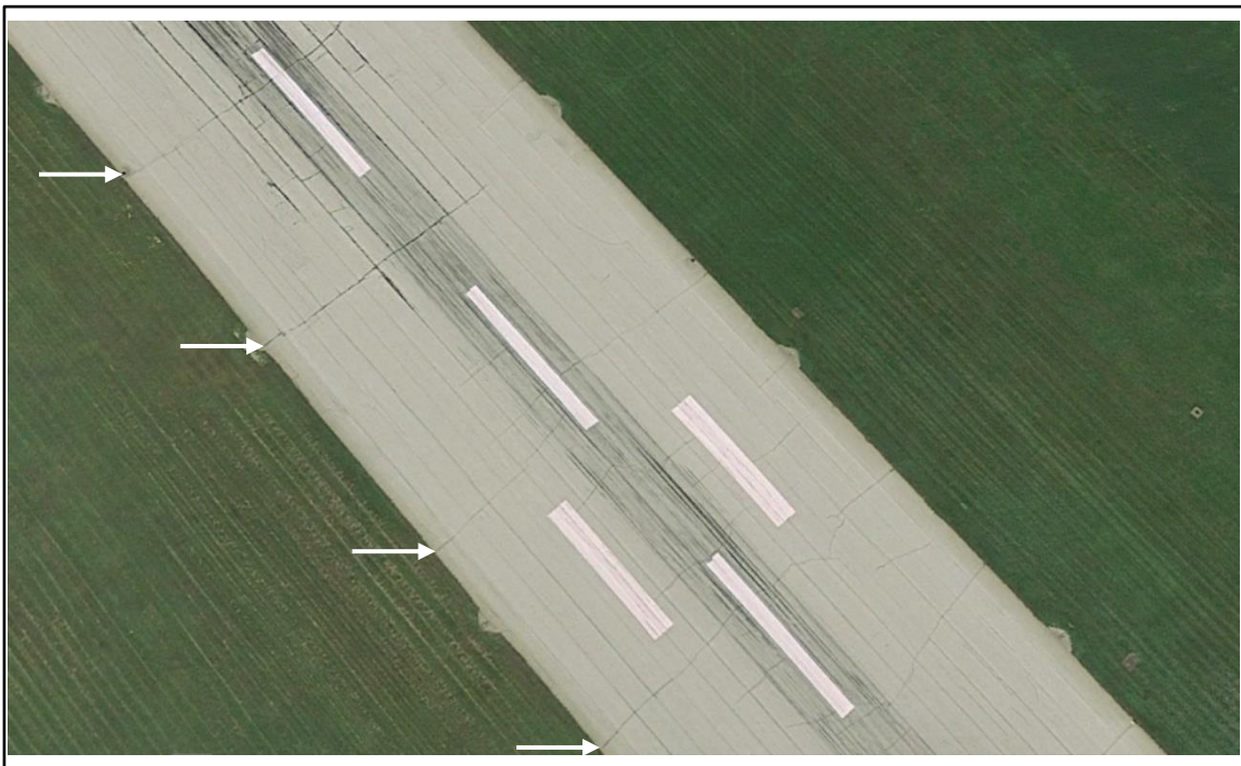
Image 2.4 Low Temp Transverse Cracking Example at YXU Airport (Google Earth Pro, 2019)
