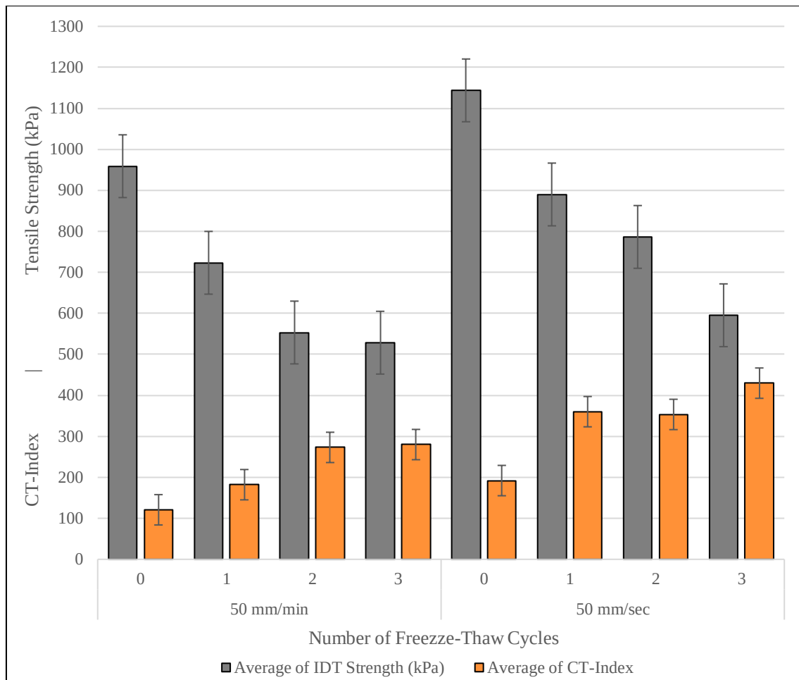
Figure 5.10 Indirect Tensile Strengths and Cracking Test Indexes
