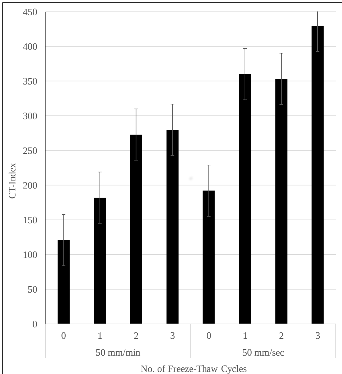
Figure B.6 Ideal CT Index Variations due to F-T Cycles and Speed of Loading
