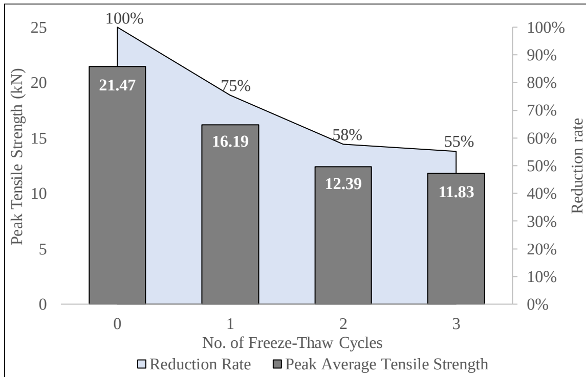
Figure 5.7 Tensile Strength versus Number of Freeze-Thaw Cycles
