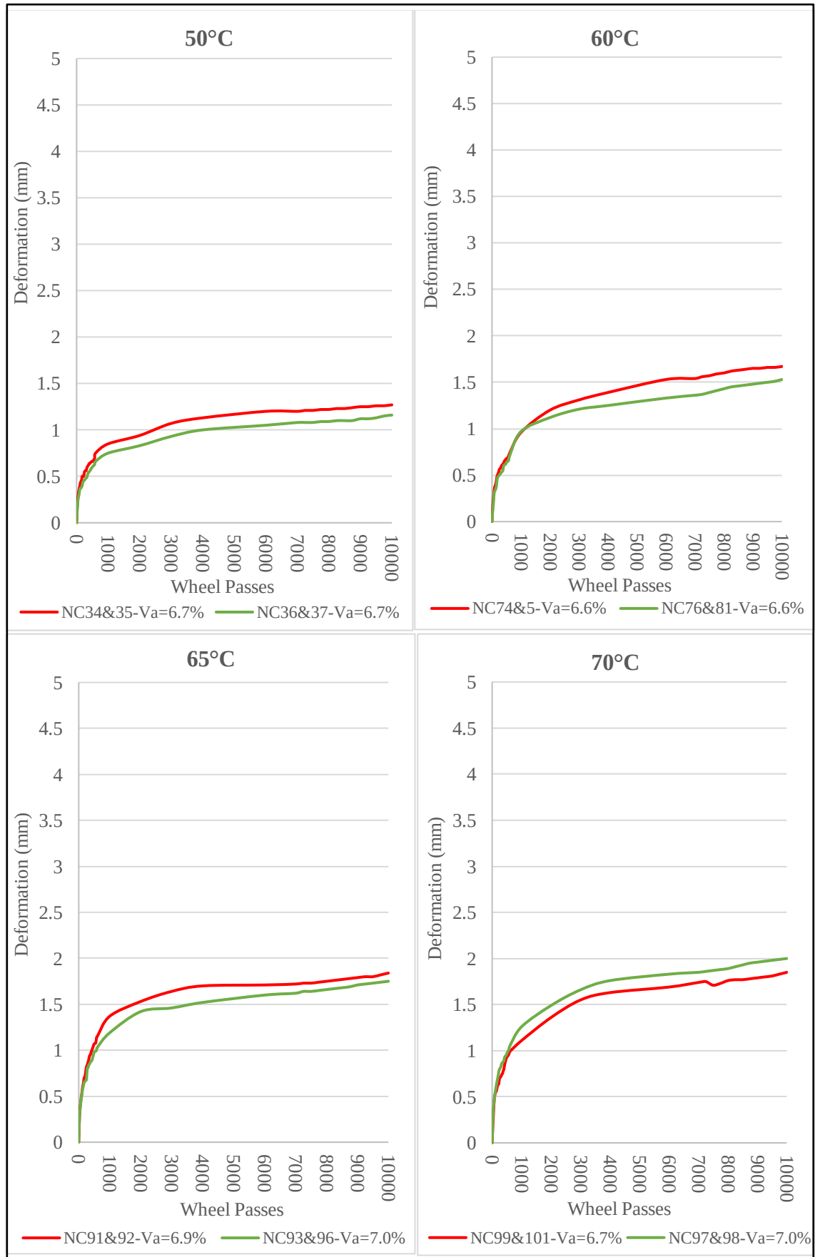
Figure B.1 Rutting Propagation versus Temperature Variation
