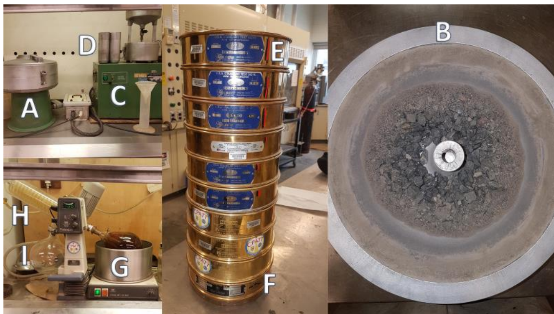
Image 5.1 Extraction and gradation tests process
