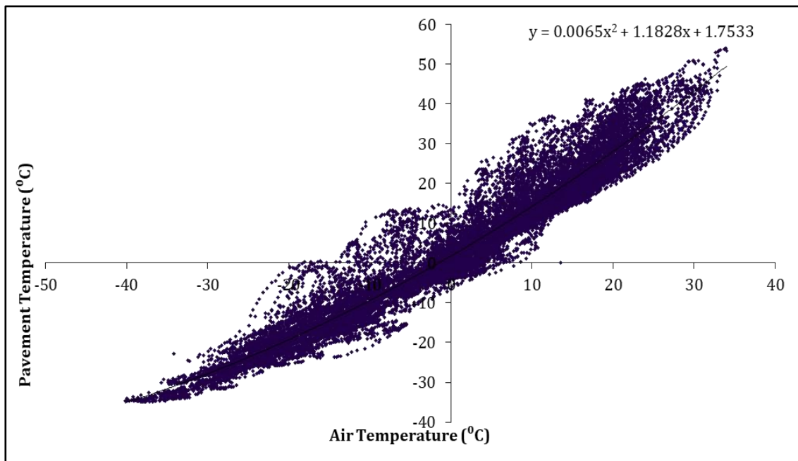
Figure 4.9 Ambient and Surface Temperature Correlation
