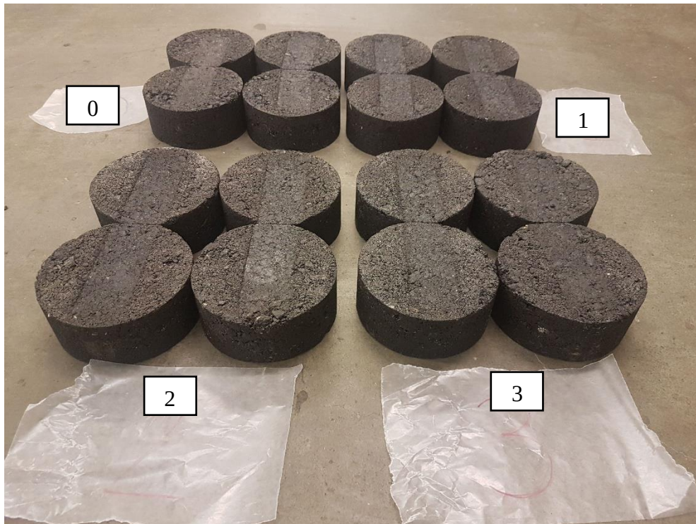
Image 5.2 Hamburg Wheel Tracking Test Samples Tested After Freeze-Thaw Cycles
