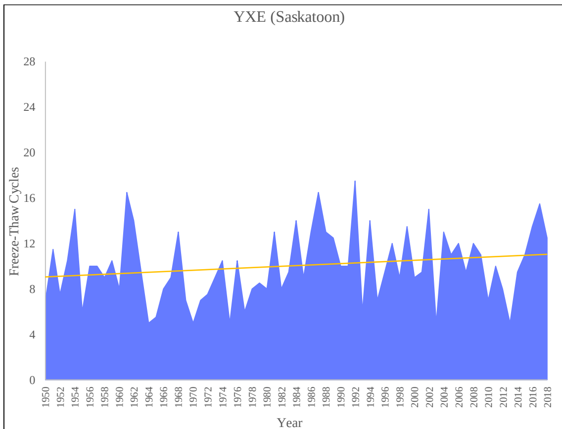
Figure A.24 Annual Freeze-Thaw Cycles for Saskatoon International Airport
