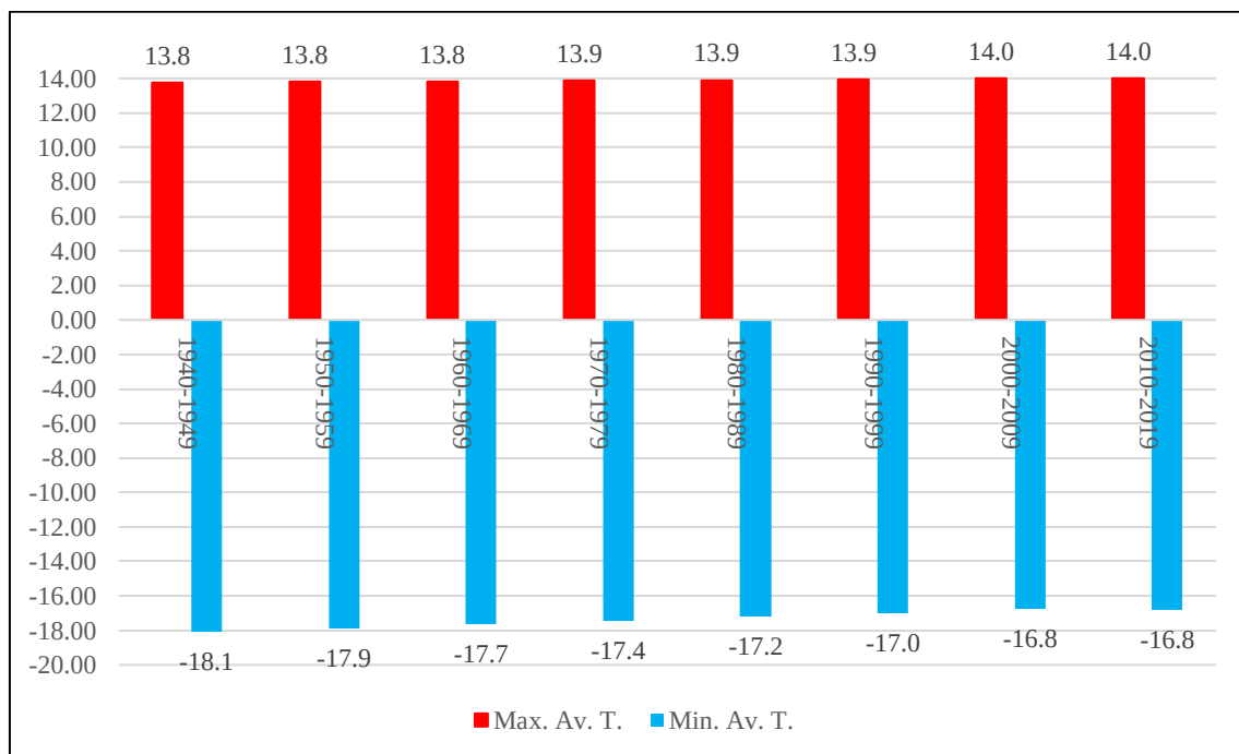
Figure A.16 Decade Average Temperature Trendlines for YXY Since 1940-1949 to 2010-2019
