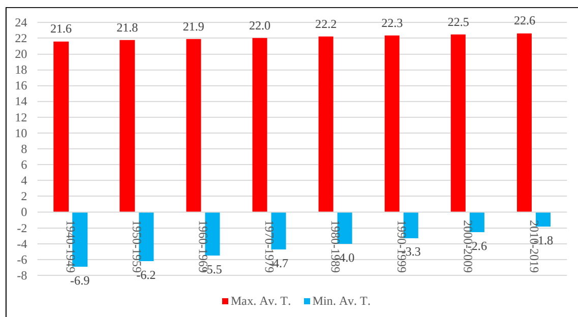
Figure A.2 Decade Average Temperature Trendlines for YYZ from 1940-1949 to 2010-2019
