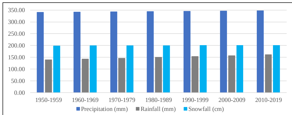
Figure A52 Annual Precip, Rainfall, and Snowfall Trends from YFB from 1950-1959 to 2010-2019
