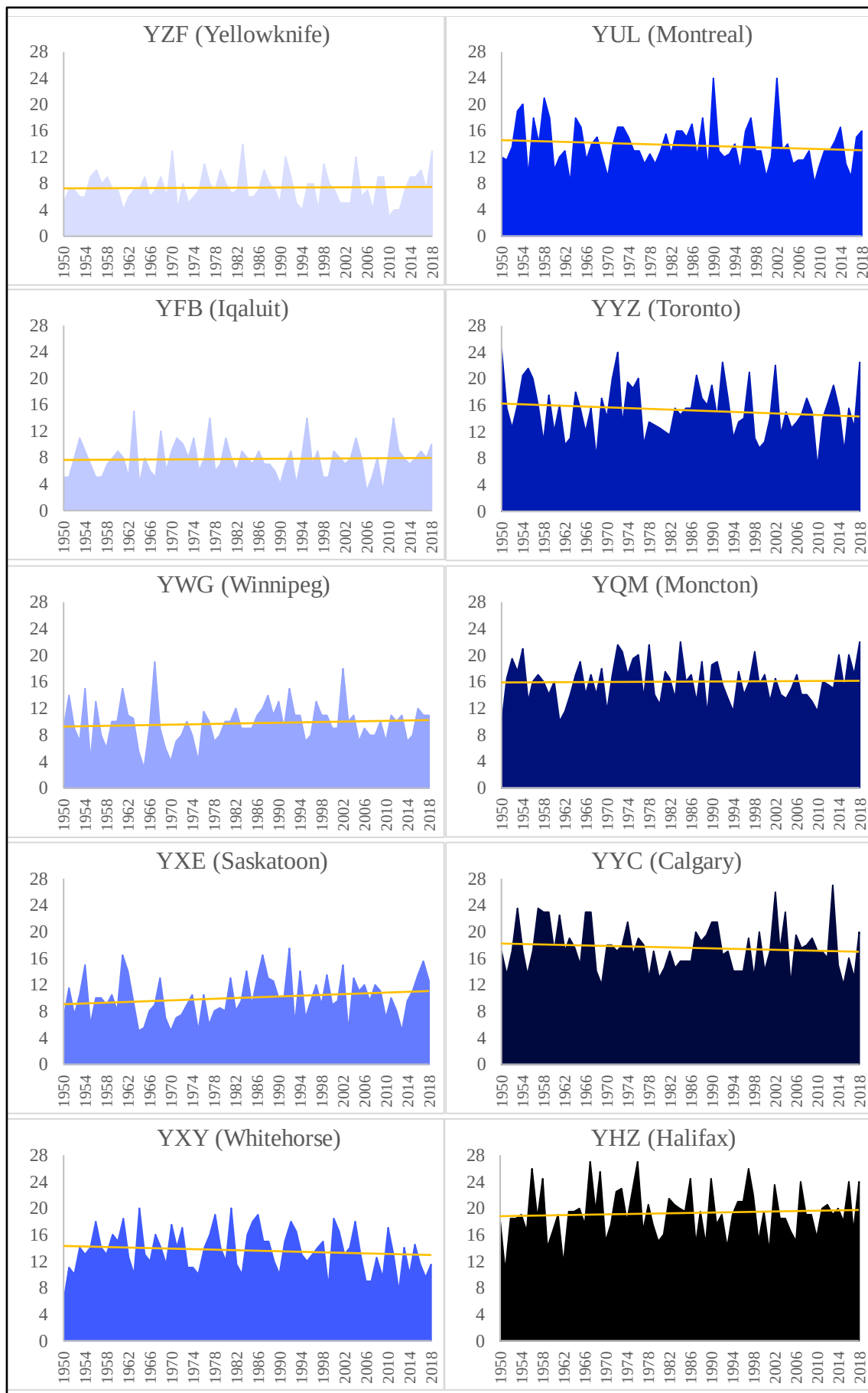
Figure 4.12 Annual Freeze-Thaw Cycles at the Selected Airports since 1950 to 2018
