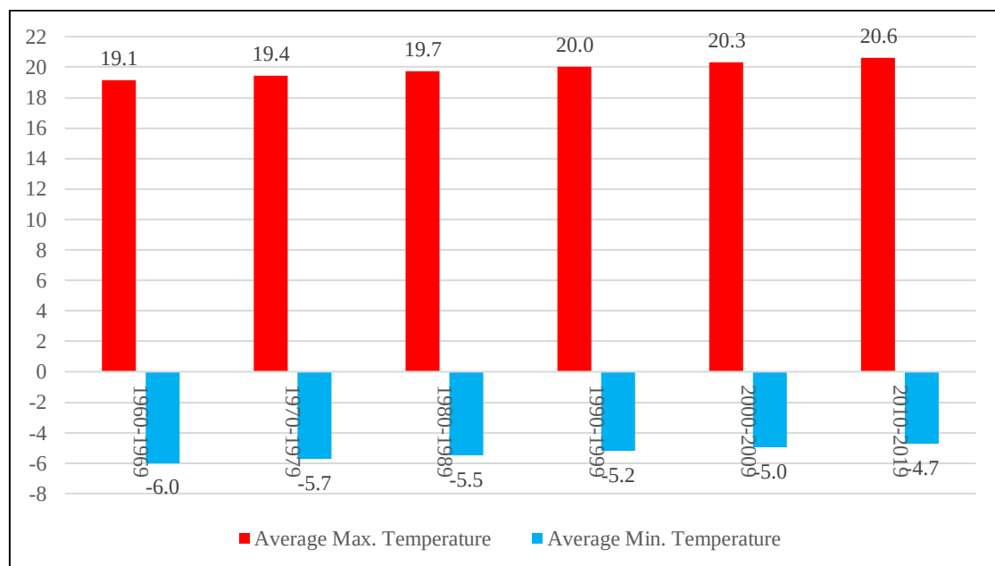
Figure A.8 Decade Average Temperature Trendlines for YHZ from 1960-1969 to 2010-2019
