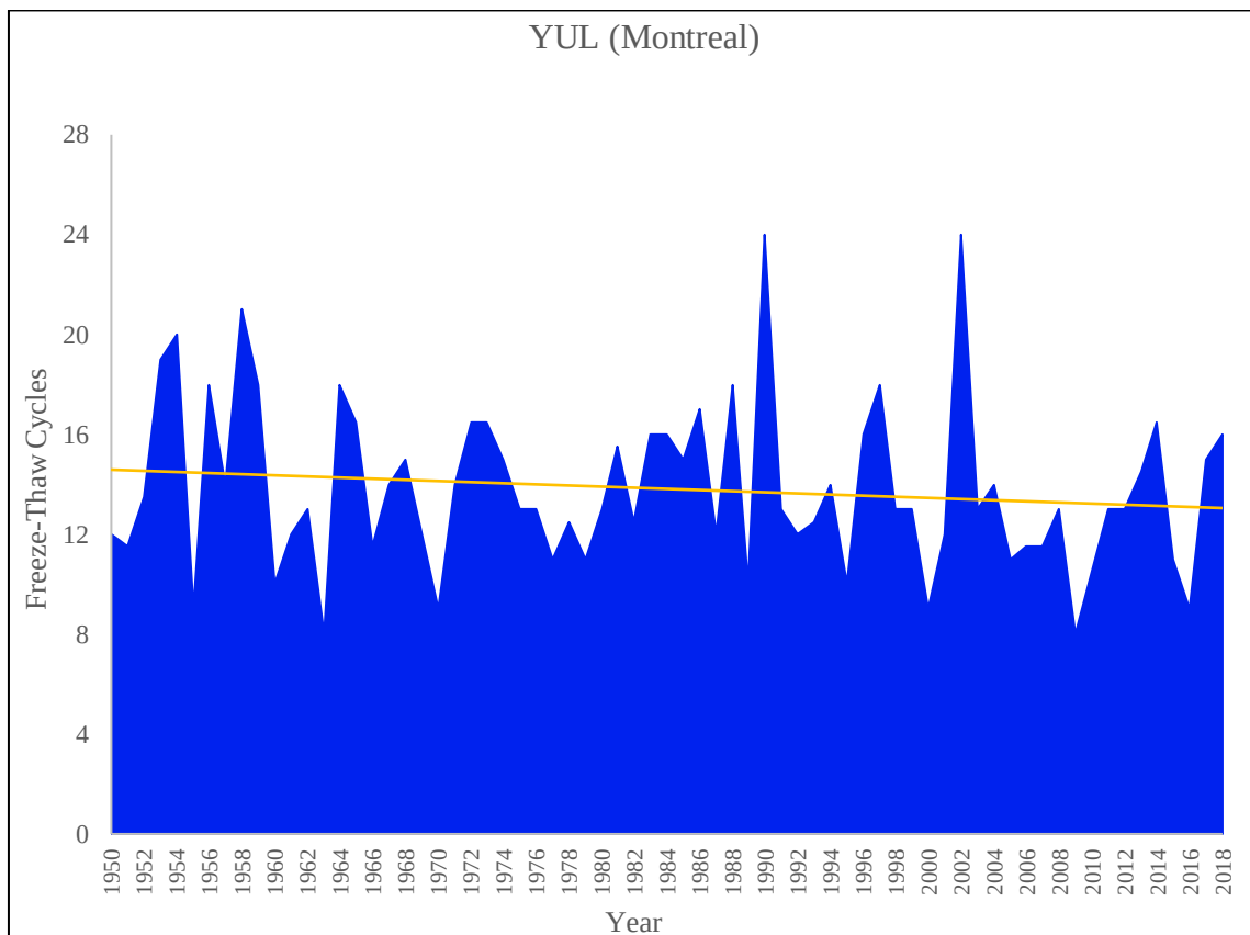
Figure A.26 Annual Freeze-Thaw Cycles for Montreal Trudeau International Airport
