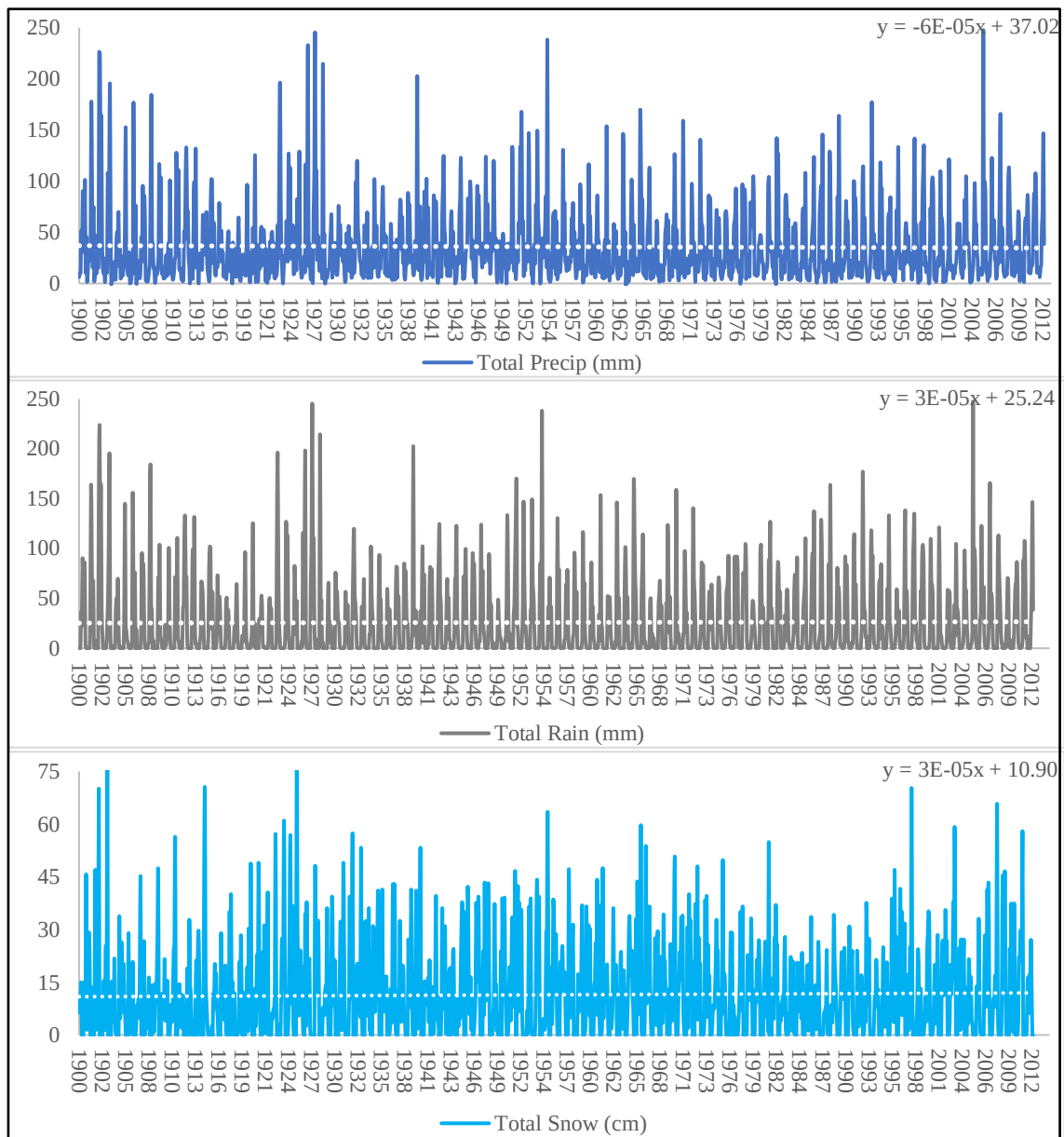
Figure A39 Annual Precipitation, Rainfall, and Snowfall for YYC from 1900 to 2012
