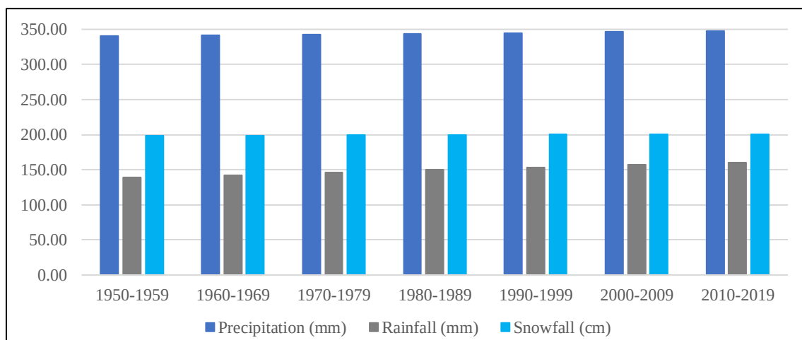
Figure A48 Annual Precip, Rainfall, and Snowfall Trends from YXY from 1950-1959 to 2010-2019
