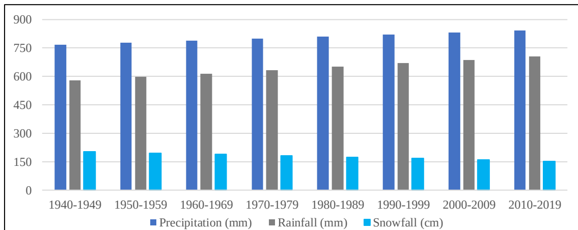
Figure A36 Annual Precip, Rainfall, and Snowfall Trends from YUL from 1940-1949 to 2010-2019
