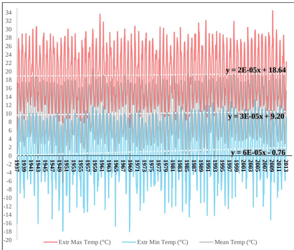
Figure 4.4 Average Minimum and Maximum Monthly Temperatures and Trendlines from 1937 to 2013 for YVR (Vancouver Airport)
