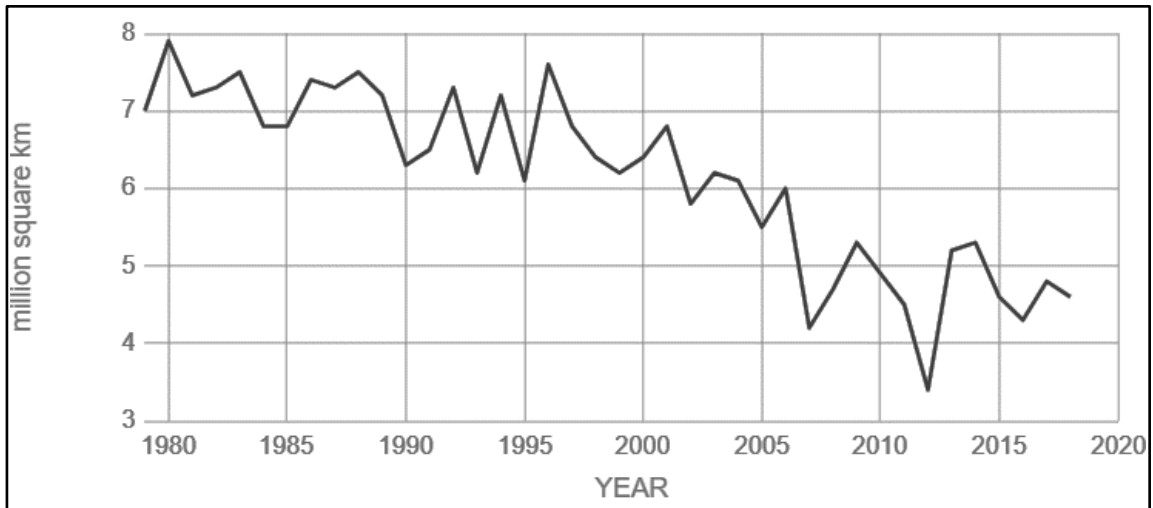
Figure 2.5 Average Arctic Sea Ice since 1980 (NSIDC/NASA, 2019)
