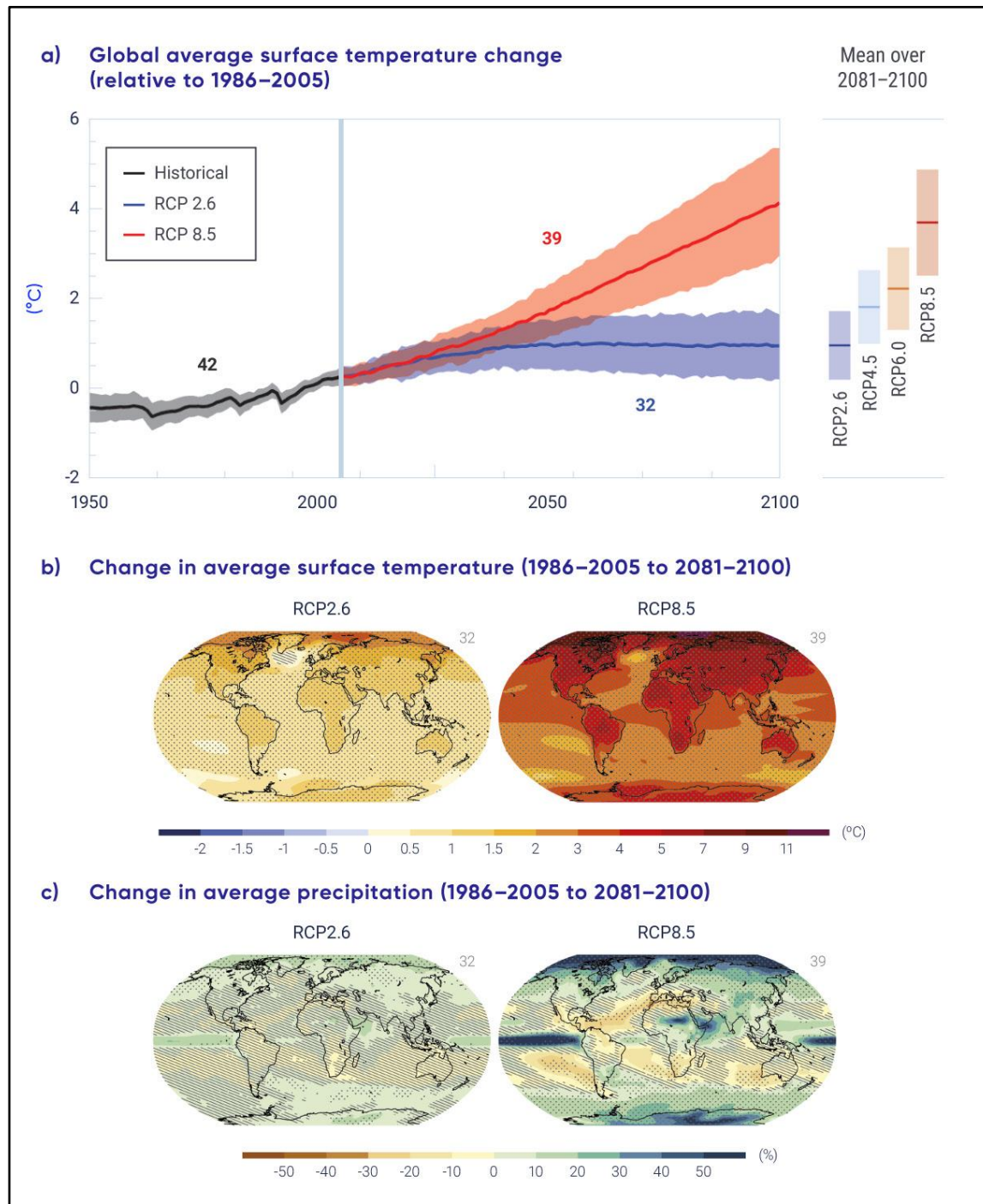
Figure 2.4 Global Climate Projections (Bush & Lemmen, 2019)
