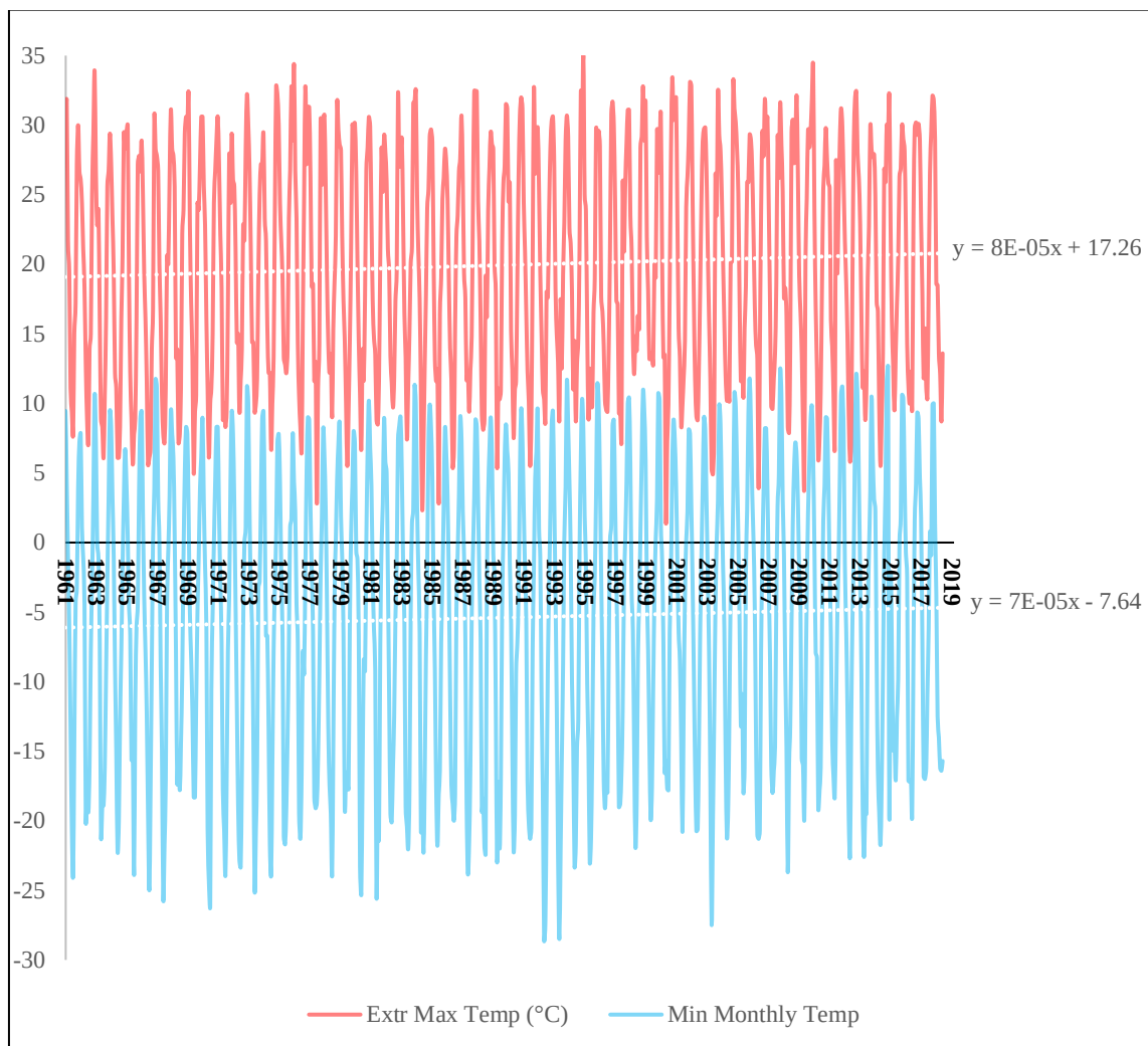
Figure A.7 Monthly Ambient Temperature at YHZ from 1961 to 2019
