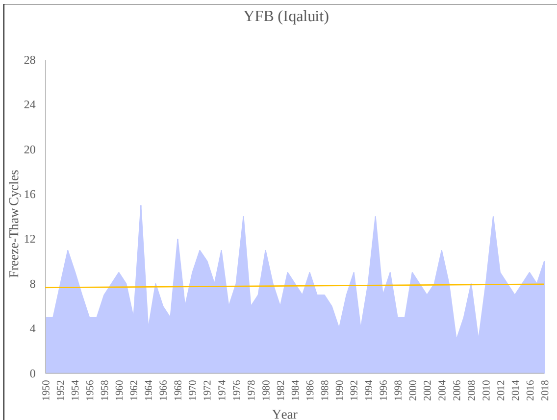
Figure A.22 Annual Freeze-Thaw Cycles for Iqaluit Airport
