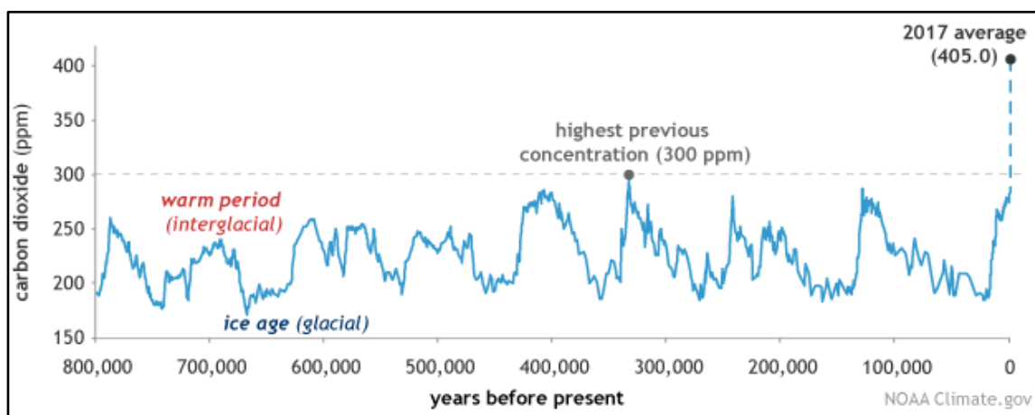
Figure 2.2 Carbon Dioxide Level during Ice Ages and Warm Period for the Past 800,000 years (National Oceanic and Atmospheric Administration, 2018)
