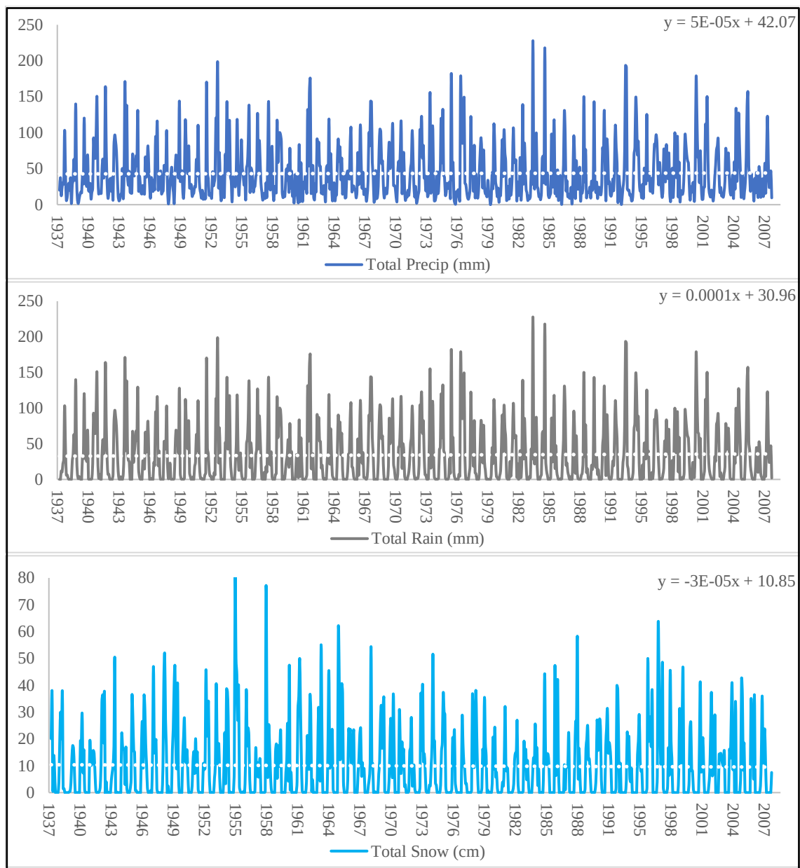
Figure A43 Annual Precipitation, Rainfall, and Snowfall for YWG from 1937 to 2007
