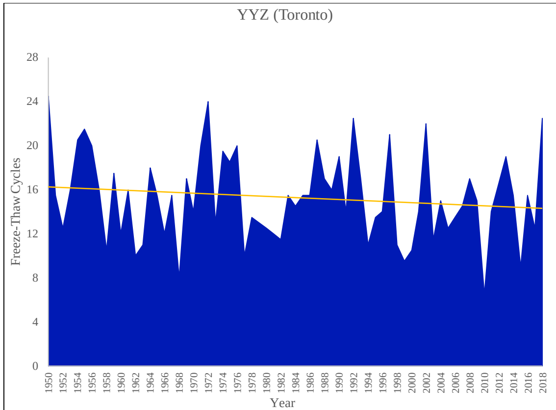
Figure A.27 Annual Freeze-Thaw Cycles for Toronto Pearson International Airport
