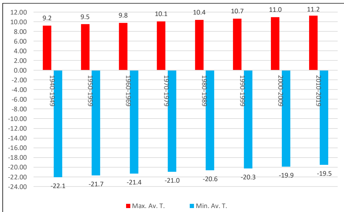
Figure A.18 Decade Average Temperature Trendlines for YXY Since 1940-1949 to 2010-2019
