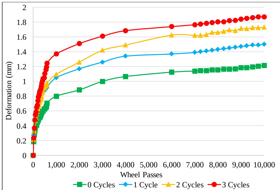
Figure 5.2 Rutting Propagation versus Freeze-Thaw Cycles
