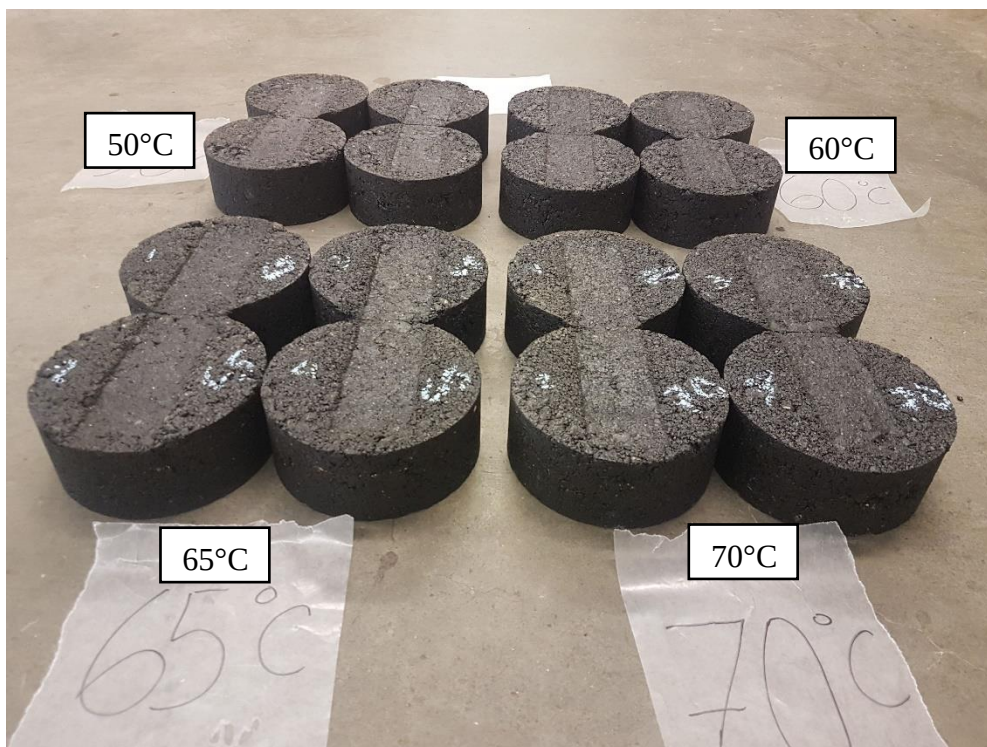
Image 5.3 Hamburg Wheel Tracking Test Samples Tested at Different Temperatures
