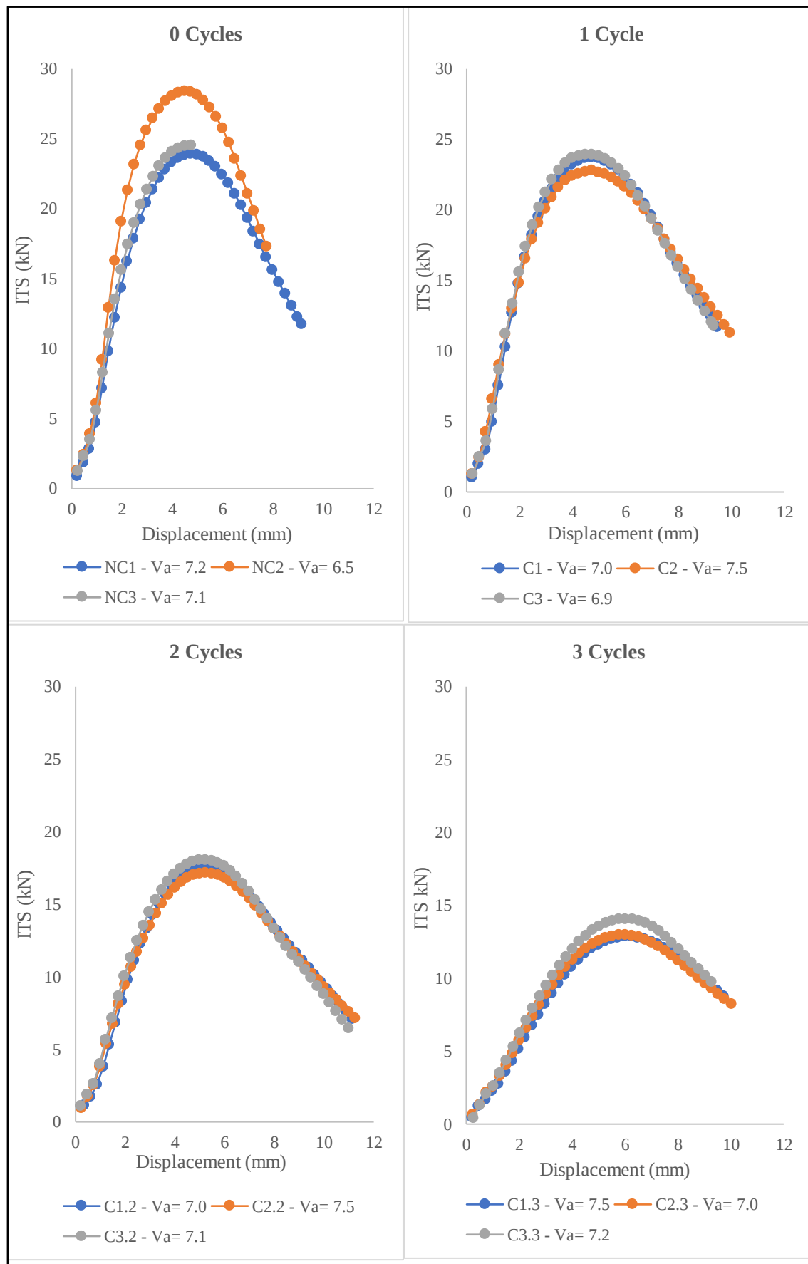
Figure B.4 ITS versus Displacement Variations due to F-T Cycles (Higher Speed of Loading)
