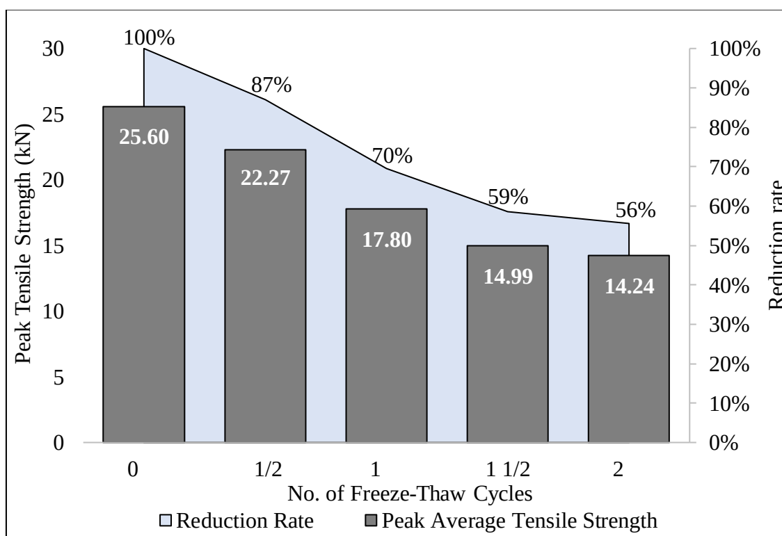
Figure 5.9 Tensile Strength with Faster Compaction and half period of Freeze-Thaw Cycles
