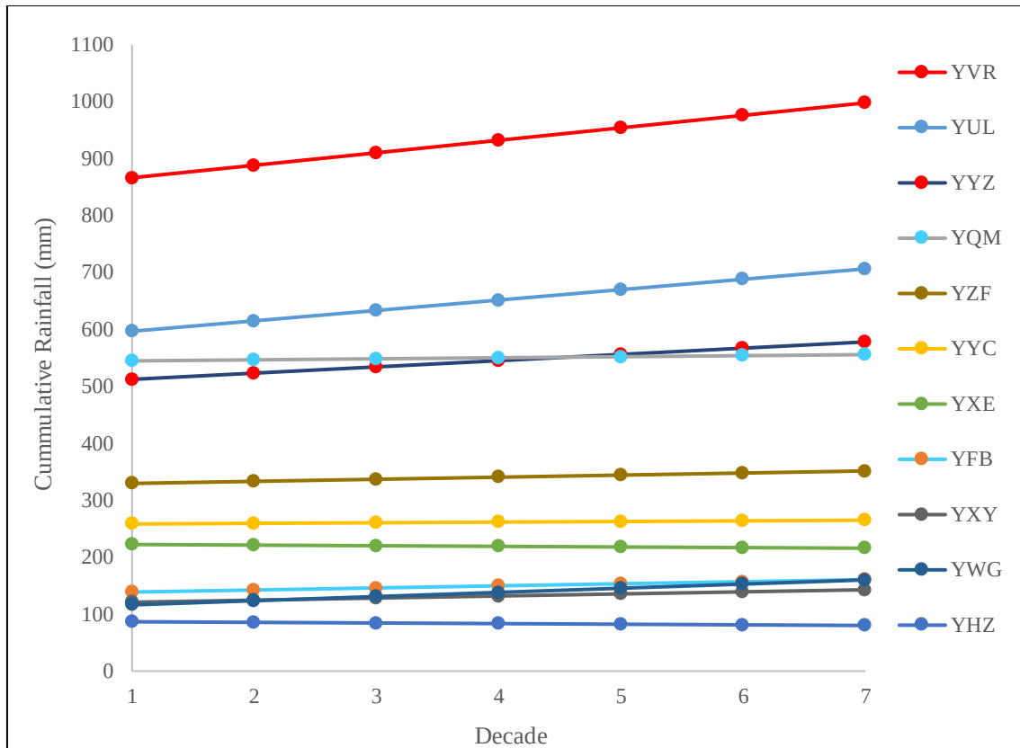
Figure 4.15 Decennial Rainfall at the Selected Airports since 1950
