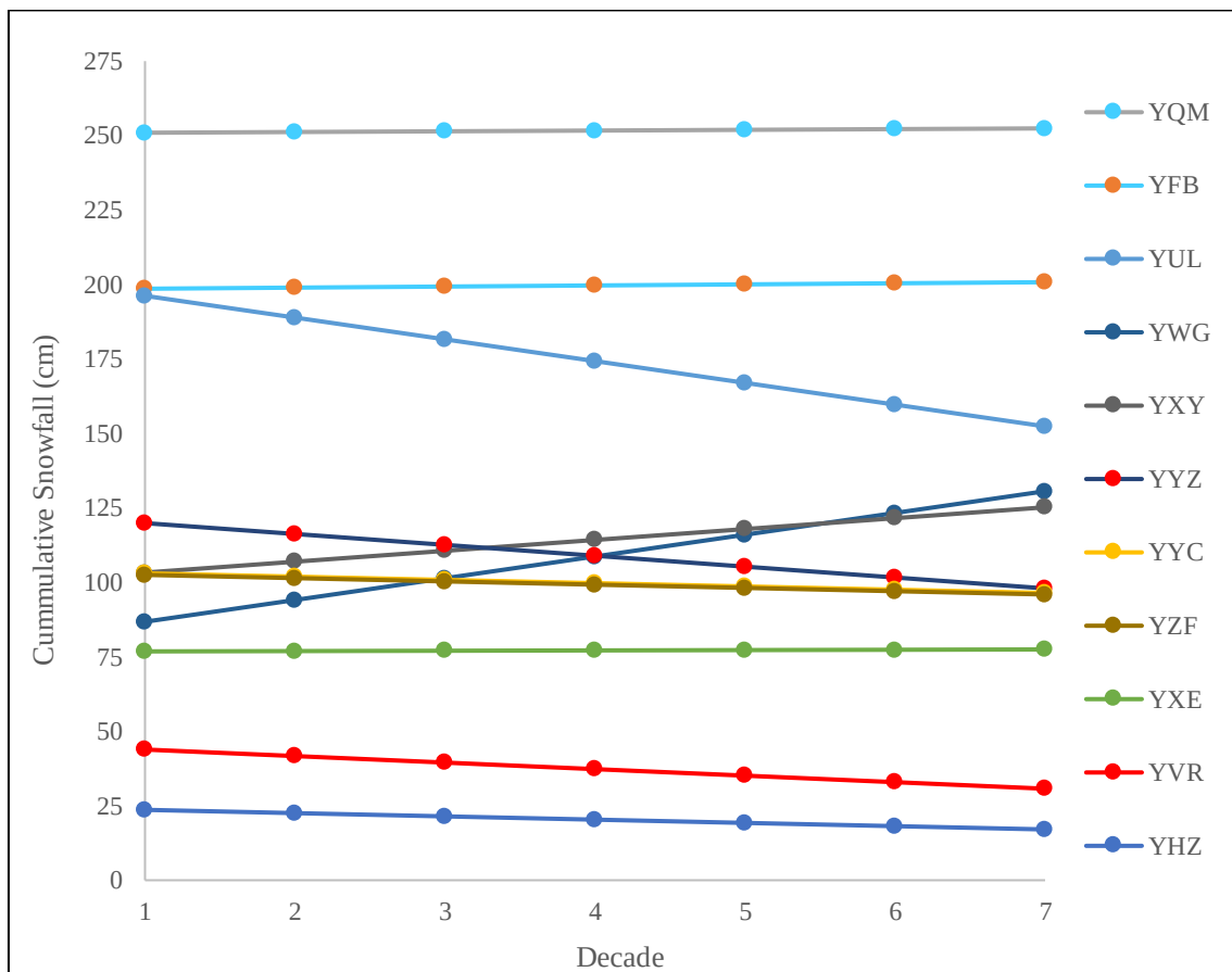
Figure 4.16 Decennial Snowfall at the Selected Airports since 1950
