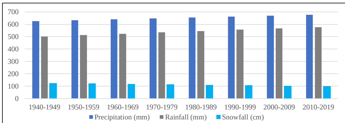
Figure A32 Annual Precip, Rainfall, and Snowfall Trends from YYZ from 1940-1949 to 2010-2019
