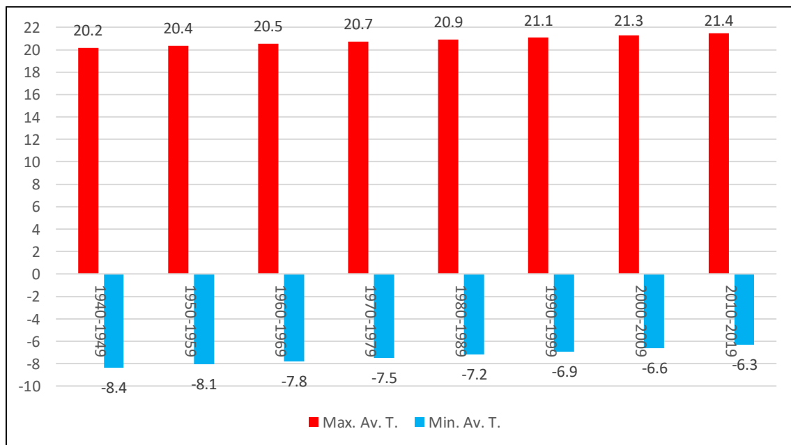
Figure A.6 Decade Average Temperature Trendlines for YUL Since 1940-1949 to 2010-2019
