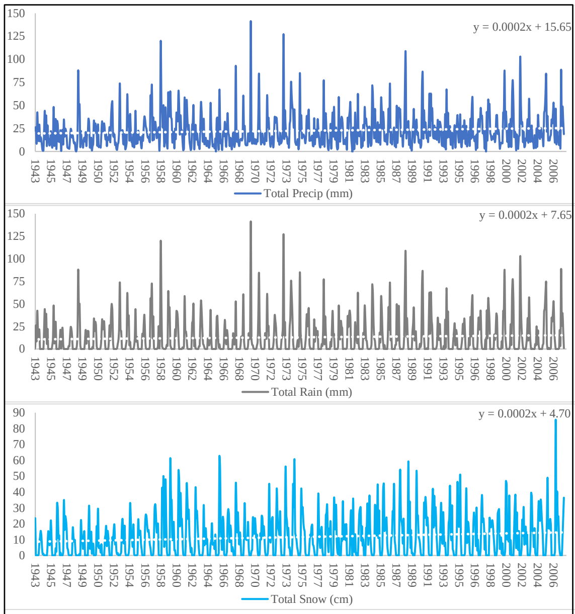
Figure A49 Annual Precipitation, Rainfall, and Snowfall for YZF from 1943 to 2006
