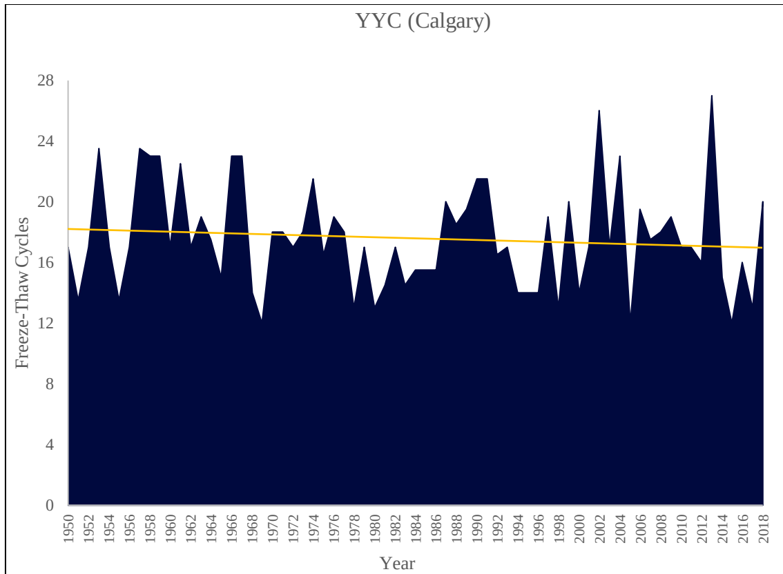
Figure A.29 Annual Freeze-Thaw Cycles for Calgary International Airport
