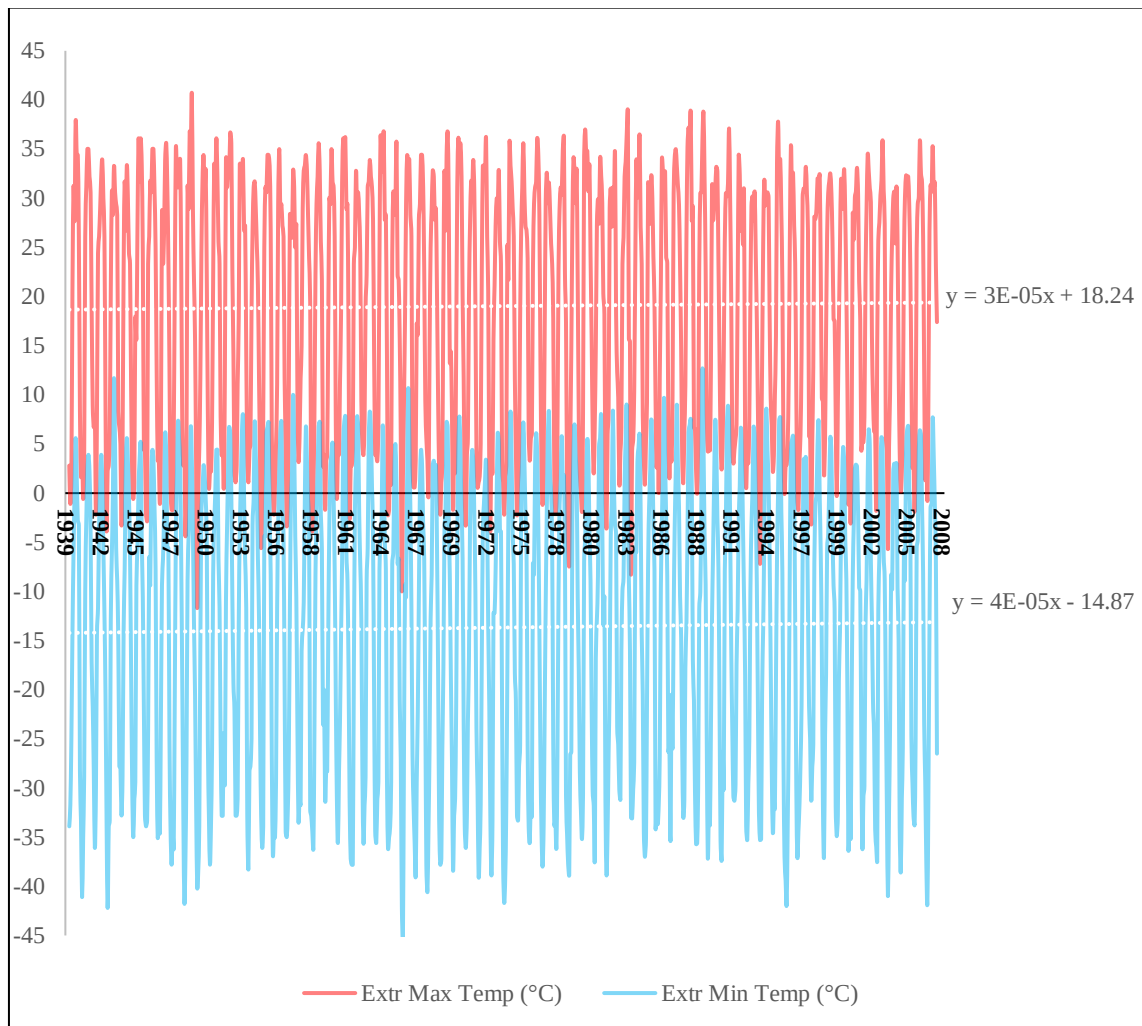
Figure A.11 Monthly Ambient Temperature at YWG from 1939 to 2008
