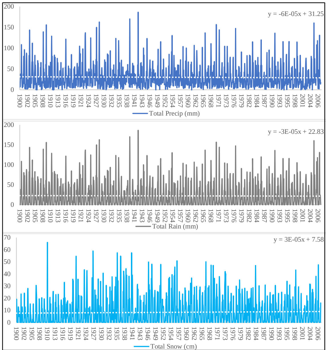
Figure A41 Annual Precipitation, Rainfall, and Snowfall for YXE from 1900 to 2006
