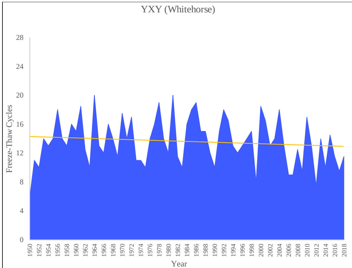
Figure A.25 Annual Freeze-Thaw Cycles for Whitehorse International Airport
