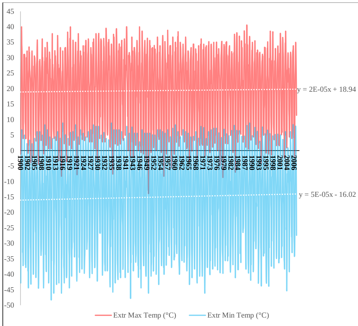
Figure A.9 Monthly Ambient Temperature at YXE from 1900 to 2006
