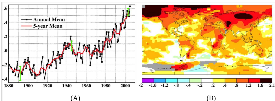
Figure 2.1 Surface Temperature Anomalies Relative to 1951-1980 (A) Global Annual Mean Anomalies. (B) Temperature anomalies for the first half decade of the 21st century (James Hansen, 2006)
