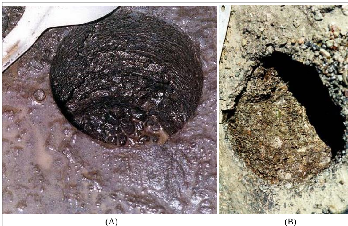
Image 2.3 Stripping | A and B are core holes showing stripping at the bottom of the layer (Pavement Interactive, 2019)
