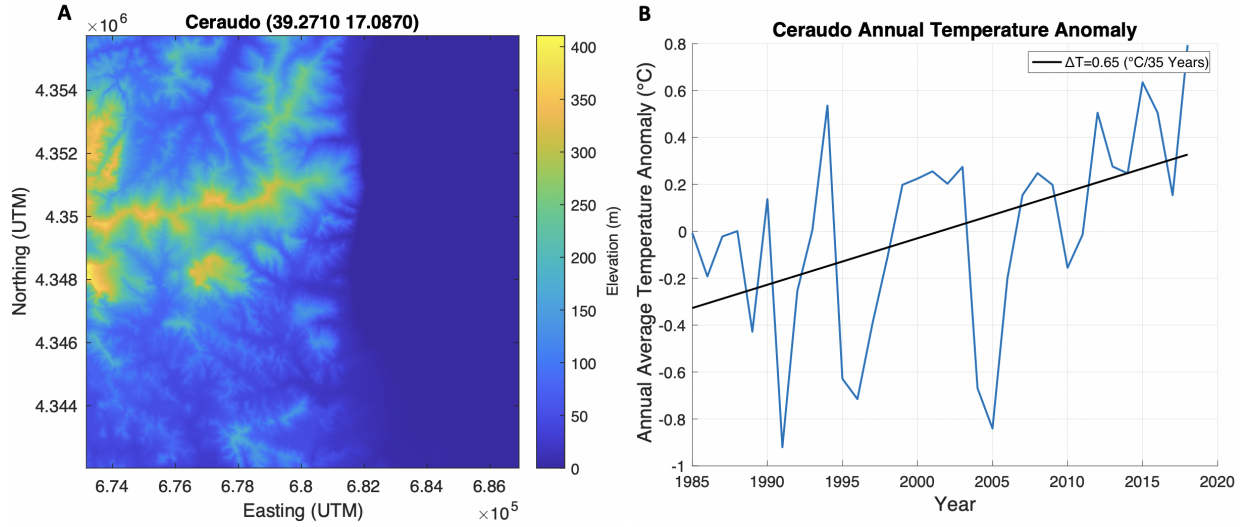
Figure 1: (A) Digital elevation model (DEM) of Tarquini et al. (2007, 2012) Ceraudo, Italy, one of the cites sampled using the Meteoblue data. Ceraudo is a costal region located in southern Italy. (B) A graph of the yearly average temperature data from 1985 to 2018 with a trend line fit to measure the warming rate of the region. Ceraudo is has increased by 0.65 °C from 1985 to 2018.
