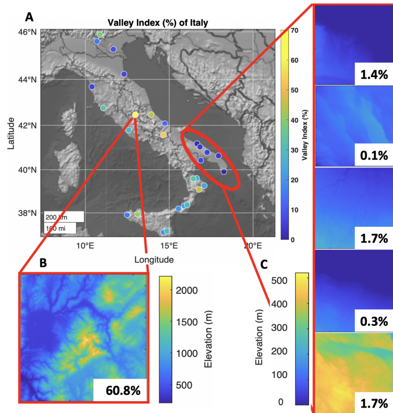
Figure 4: (A) Regions identified as anomalies in (Figure 4). The high valley index is Terminillo Mountain, which has a valley index of 60.8 percent (B) and is located in the Abruzzi Apennine region of Italy. Meanwhile the regions with the higher warming rate than those in similar latitudes with a low valley index (C) are all located in the Apulia Region (from top to bottom: Brindisi, Darioratta, Frantoio De Carlo, Olio Intini, and Tre Colonne) where the terrain is relatively flatter than the rest of Italy.
