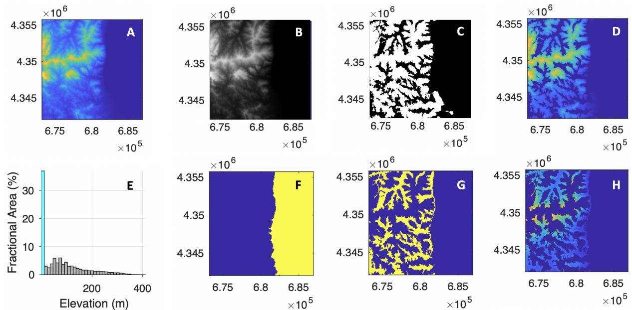
Figure 2: Algorithm used to compute the percentage of valleys at Ceraudo (coordinates in UTM). With the topography data (A), the algorithm converts the data into a gray scale image (B) uses the adaptive threshold (C) to identify the lower regions (D). In order to remove the ocean from the valley index, a histogram of the elevation data is calculated (see Equation 3 ). (E) Ceraudo has a flat ground percentage of 36.93 percent of an elevation of about 5.7 m, so a flat ground filter was applied (F) and subtracted from the original filtered area (G to H). The calculated valley index for Ceraudo is 22 percent.
