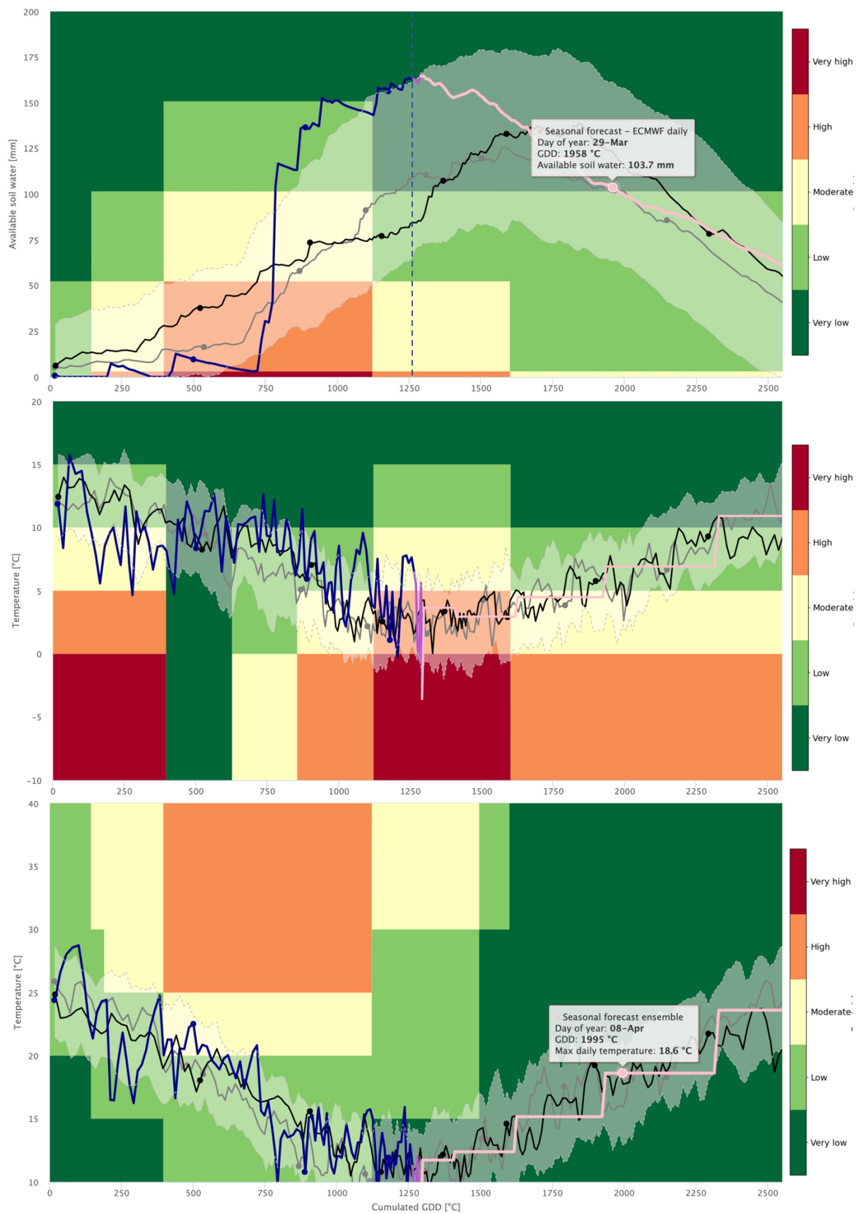
Figure 5: Example of crop weather risk monitoring and prediction diagram for drought risk (top), frost risk (centre) and heat risk (bottom). Winter wheat, growing season October-May. Location (lat, lon): (40.0, 16.6). Base temperature 0°C. Soil capacity 200 mm. Water stress: available soil water < 3 mm. Frost: daily min temperature < 0°C. Heat: daily max temperature > 30°C. Dotted lines: climatic average 1985-2020 +/- standard deviation.
