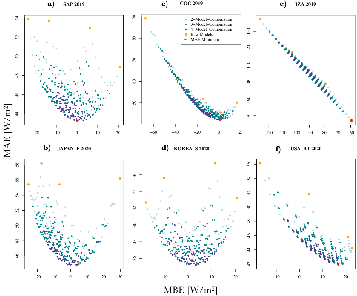
Figure 4: Scatterplots of MAE and MBE of all multi-model combinations. On the left (a and b) and in the middle (c and d), stations are shown where M4-combinations achieve the lowest MAE . The best combinations as well show low MBE 's. On the right (e and f), stations are illustrated which form exemptions. For IZA 2019, no multi-model could lower the MAE . USA_BT shows, that low MAE 's might as well mean unsatisfying MBE 's.
