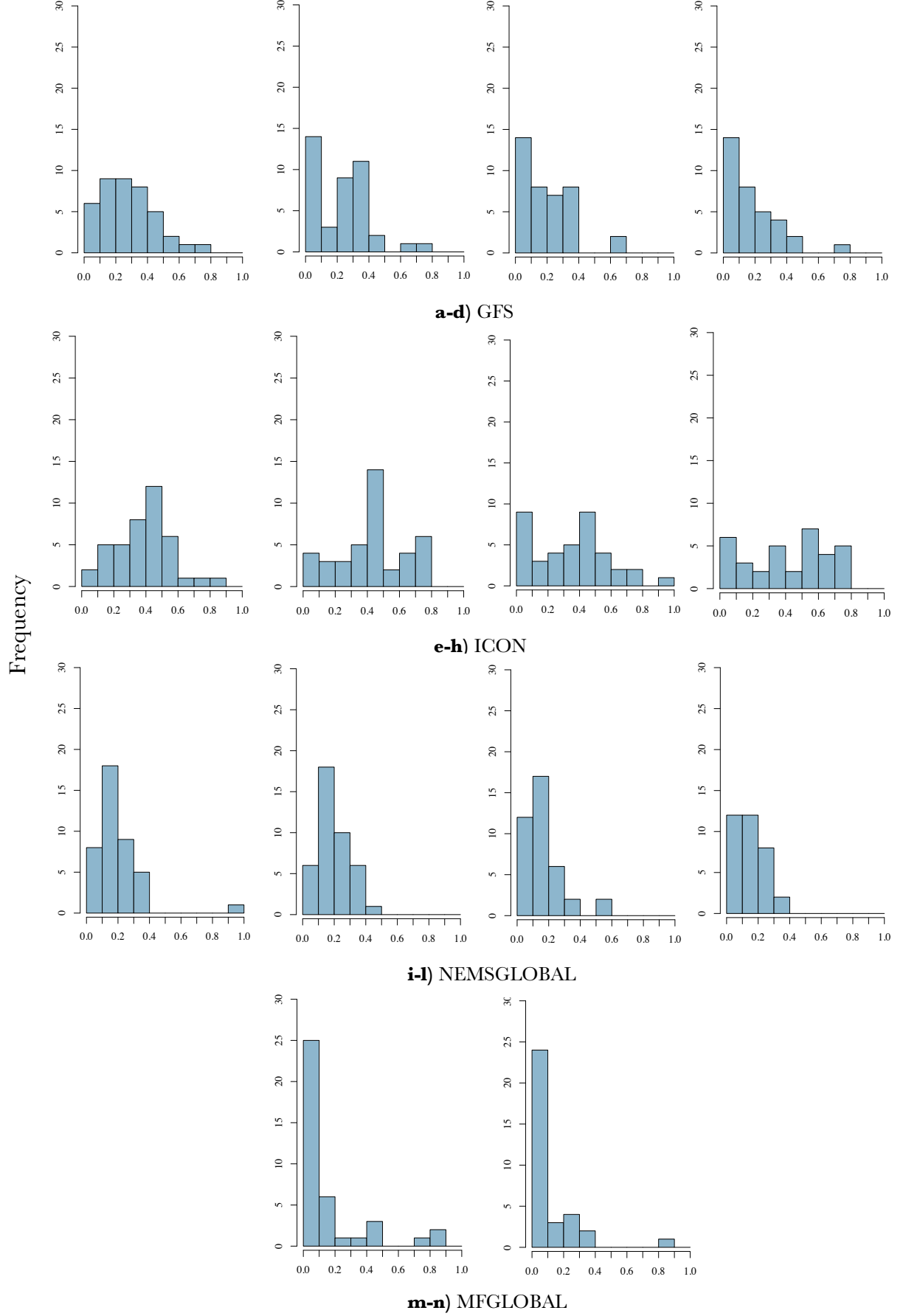
Figure 6: Histograms showing how each model was weighted for each station to achieve the lowest MAE . The x-axis describes, how high the models were weighted, the y-axis represents the number of stations affected. From left to right, BSRN 2018, BSRN 2019, WRDC 2018 and WRDC 2020 are shown. M) and n) are an exemption and show only results for BSRN 2018 (m) and WRDC 2020 (n).
