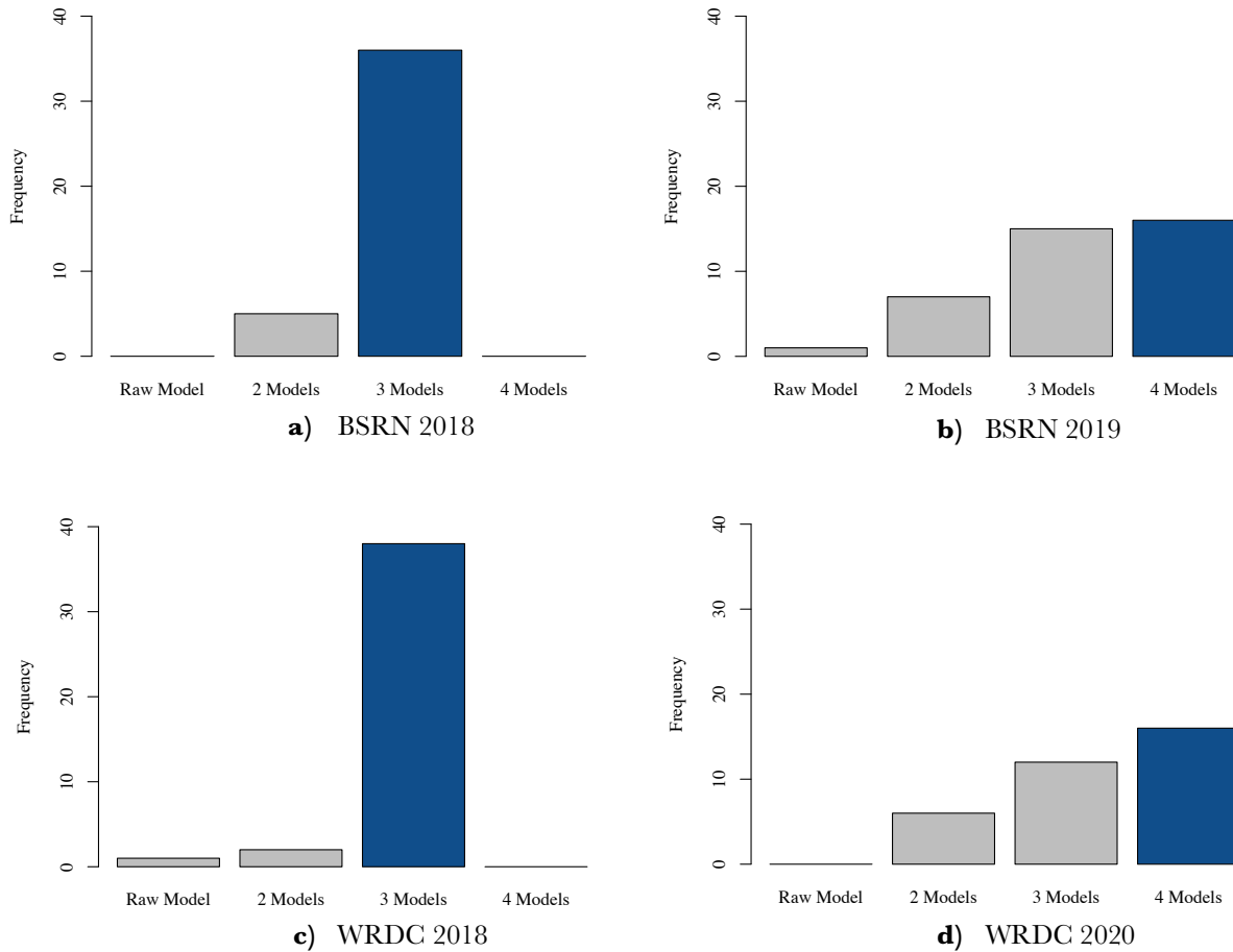
Figure 5: Barplots showing how often raw models, M2, M3 or M4-combinations achieved the lowest MAE per dataset and year.
