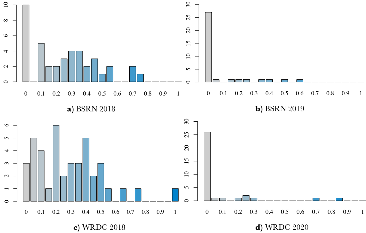
Figure 7: The number of overlapping combinations within the 20 best MAE 's of each quarter of every station. The x-axis represents an index describing the relative amount of overlapping combinations out of all 20 best combinations within all four seasons of one station. The y-axis shows, how many stations are affected. Note, that the resolution of the y-axes between the four bar plots differs.
