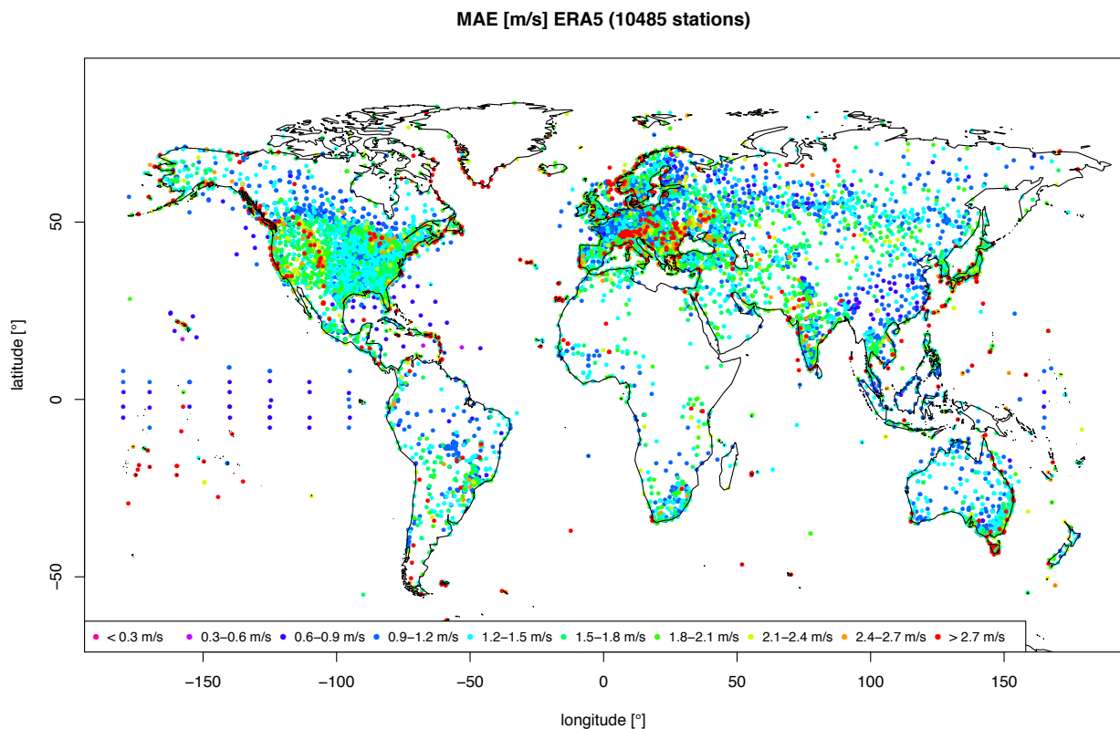
Fig. 4: MAE [ \text{m s}^{-1} ] of the 10 m wind speed of the reanalysis model ERA5 (not available as forecast) used for long term historical analysis. Verification is based on all hourly data of the year 2017.
