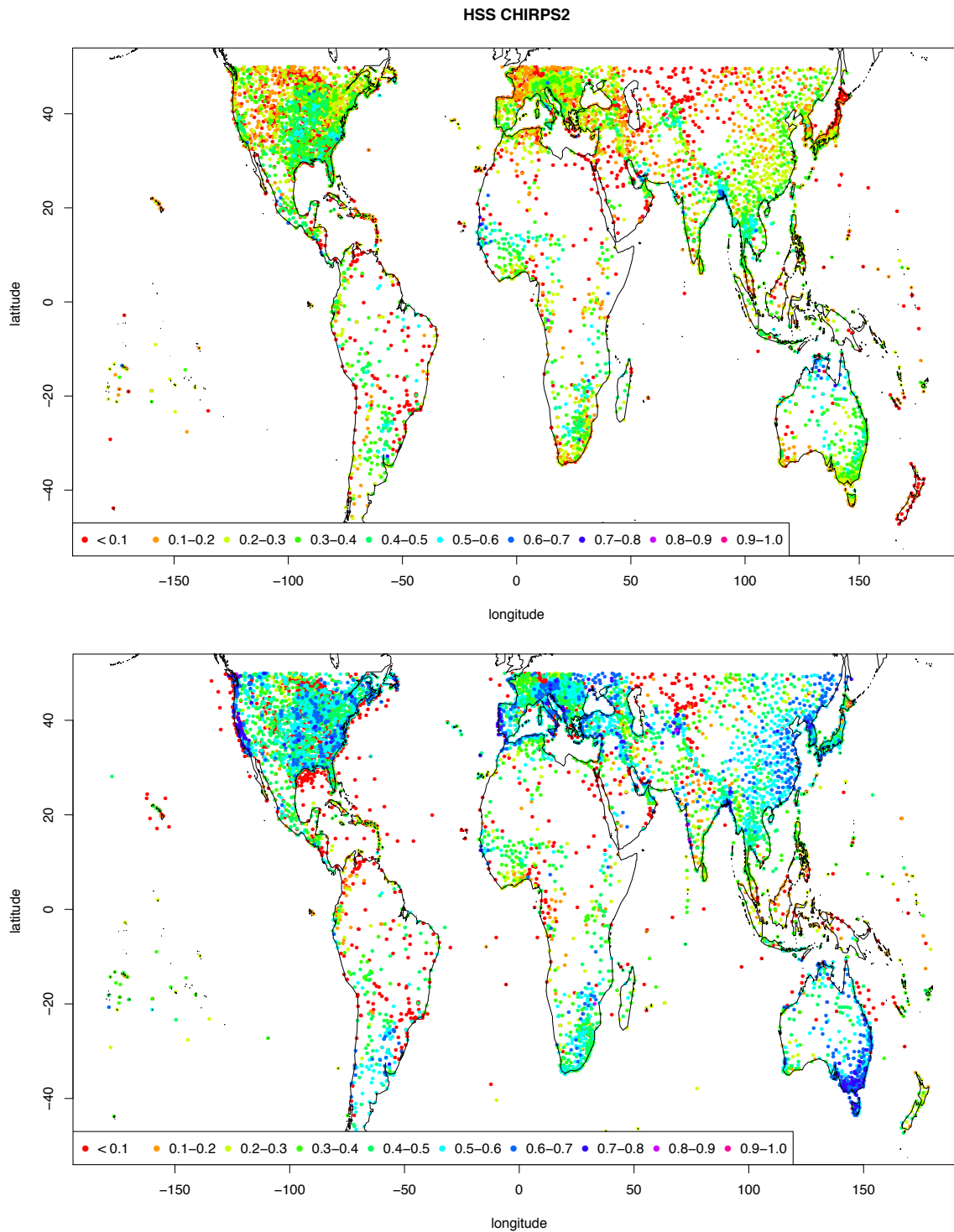
Fig. 8: Heidke Skill Score (HSS) for precipitation events of >1mm/day for the satellite observation CHIRPS2 (not available as forecast) used for long term historical analysis (top) and the meteoblue Learning Multi-Model (MLM) used in forecasts (bottom). Verification is based on all daily data of the year 2017.
