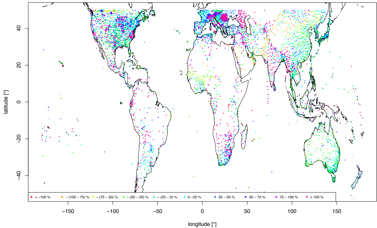
Fig. 9: MPE [%] for the meteoblue Learning Multi-Model (MLM) used in operational forecasting. Verification is based on all daily data of the year 2017.
