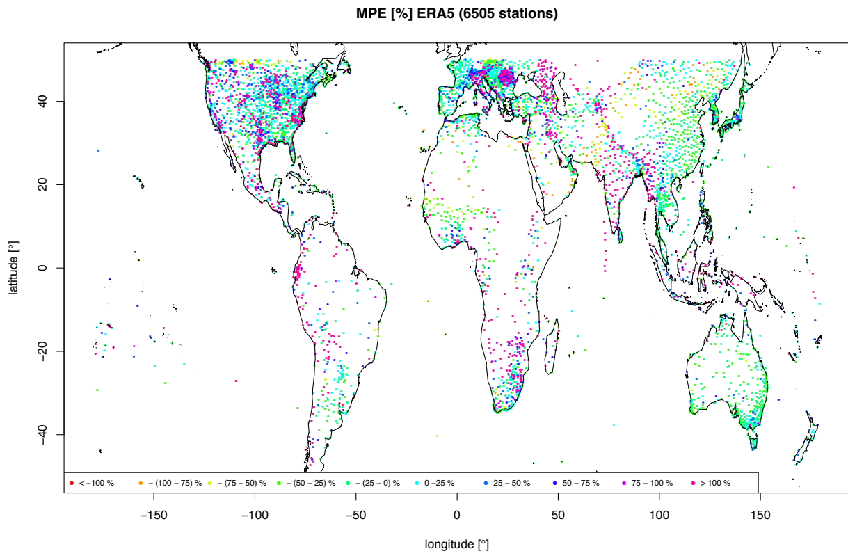
Fig. 11: MPE [%] for the historical reanalysis model ERA5. Verification is based on all daily data of the year 2017.
