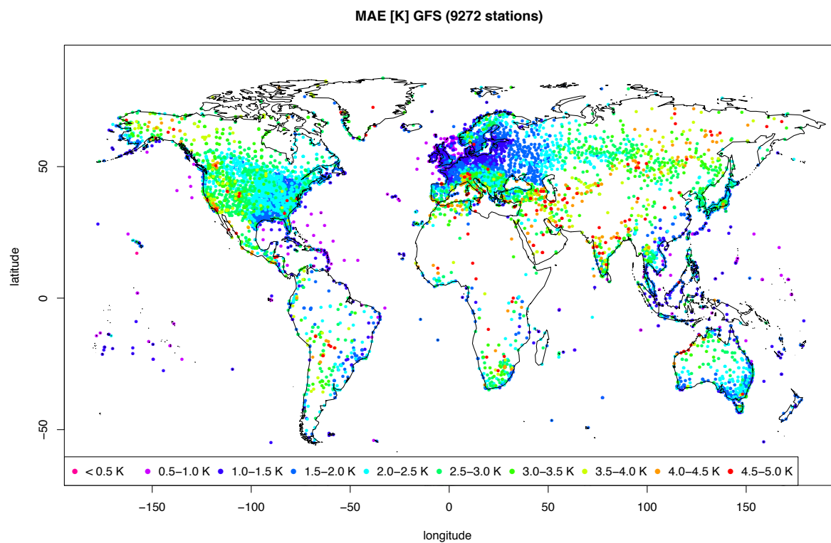
Fig. 14: MAE [K] of the numerical weather forecast model GFS. Verification is based on all hourly data of the year 2017.
