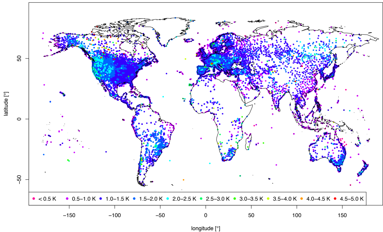
Fig. 2: MAE [K] of the 2 m air temperature of the meteoblue Learning Multi-Model (MLM) used in operational weather forecast . Verification is based on all hourly data from September and October 2018.
