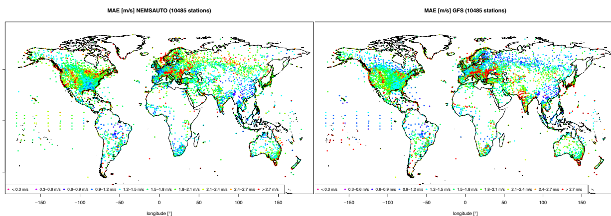
Fig. 6: MAE [ \text{m s}^{-1} ] of the 10 m wind speed of the 'stand-alone' model output as computed by meteoblue NEMS (left) and GFS (right), respectively. Verification is based on all hourly data of the year 2017.
