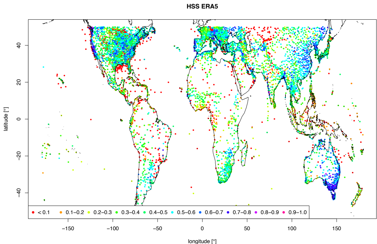
Fig. 7: Heidke Skill Score (HSS) for precipitation events of >1mm/day for the reanalysis model ERA5 (not available as forecast) used for long term historical analysis. Verification is based on all daily data of the year 2017.
