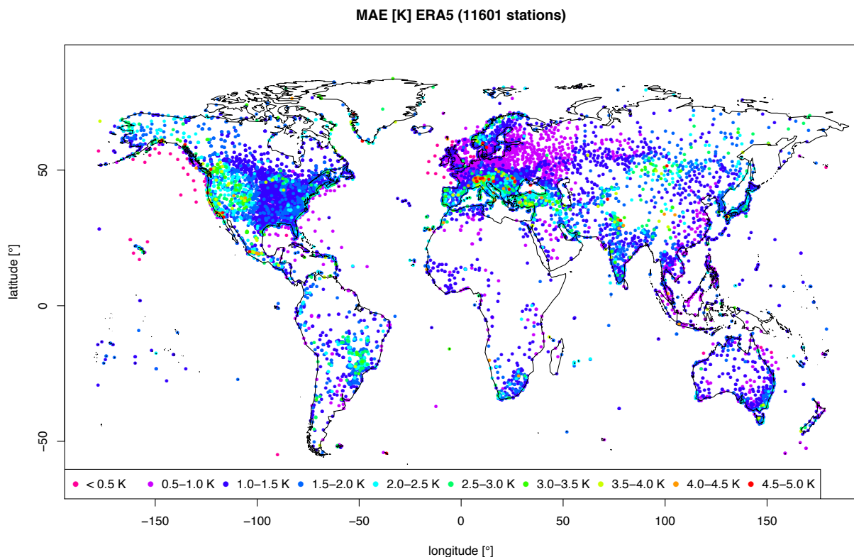
Fig. 1: MAE [K] of the 2 m air temperature of the ERA5 reanalysis (not available as forecast) used for long term historical analysis. Verification is based on all hourly data of the year 2017.
