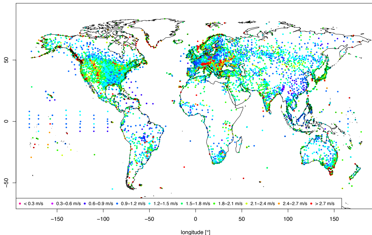
Fig. 5: MAE [ \text{m s}^{-1} ] of the 10 m wind speed of the meteoblue multi-model mix used in operational weather forecast . Verification is based on all hourly data of the year 2017.
