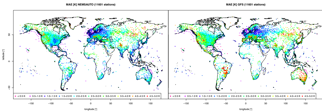
Fig. 3: MAE [K] of the 2 m air temperature of the 'stand-alone' model output as computed by meteoblue NEMS (left) and GFS (right), respectively. Verification is based on all hourly data of 2017.
