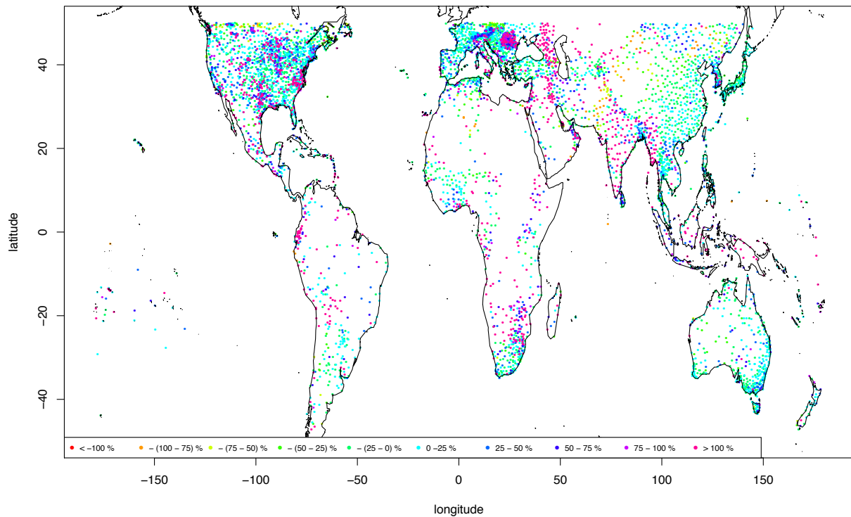
Fig. 10: MPE [%] for the historical meteoblue multi-model mix. Verification is based on all daily data of the year 2017.
