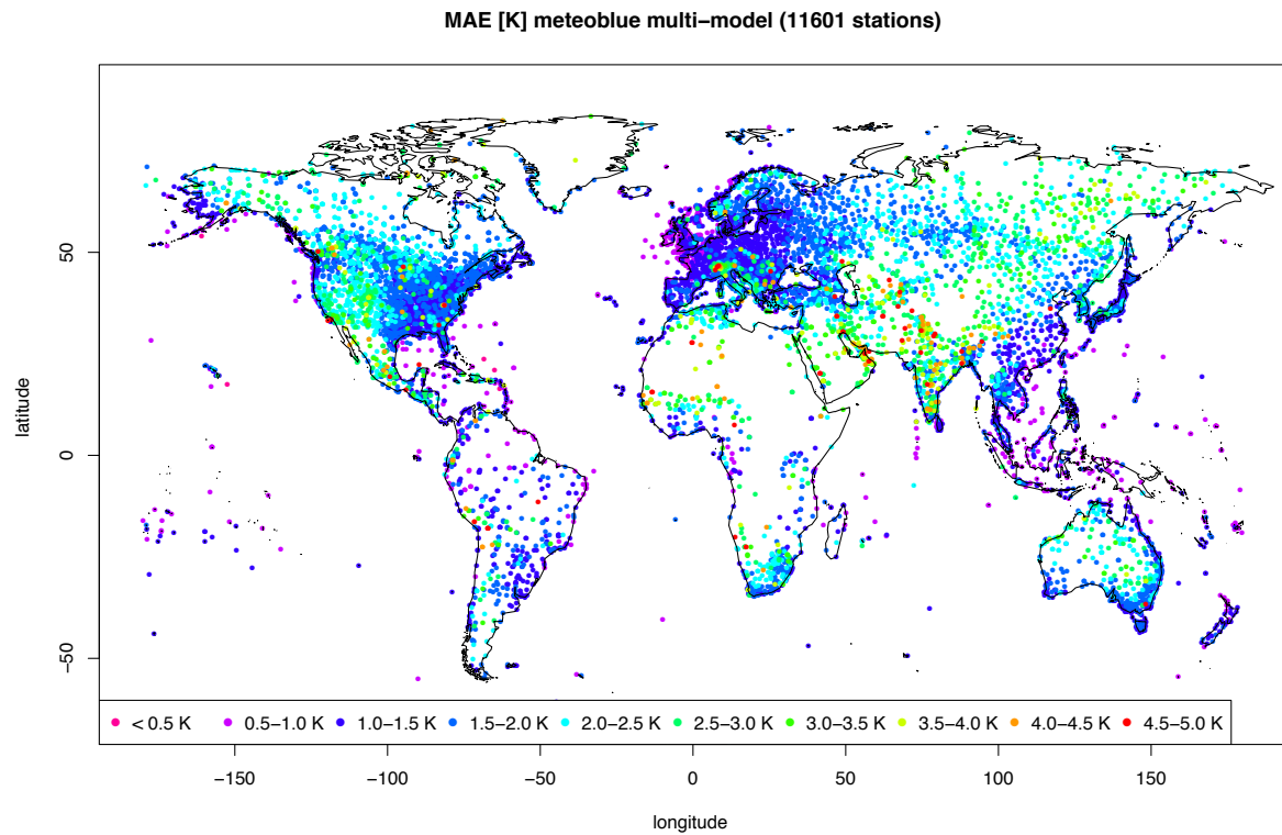
Fig. 13: MAE [K] of the meteoblue multi-model mix used in operational forecast. Verification is based on all hourly data of the year 2018.
