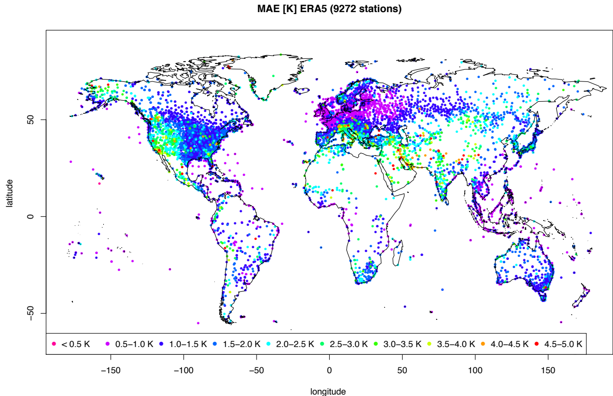
Fig. 12: MAE [K] of the reanalysis model ERA5. Verification is based on all hourly data of the year 2017.
